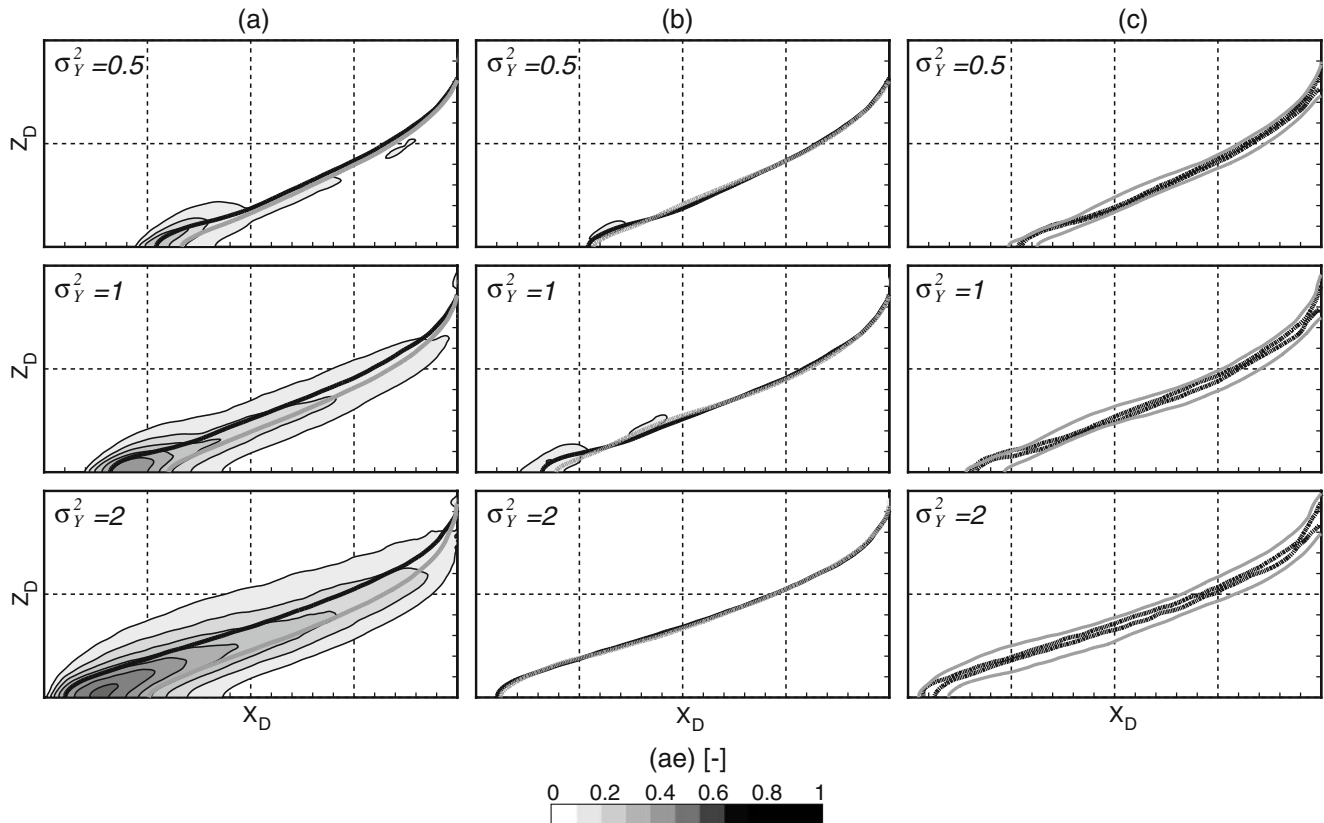
Fig. 12 Comparison between 2D, 2D* and 3D anisotropic cases ( l_x=0.12 , l_y = l_z=0.04 ) for different levels of \ln(K) variances. a 3D ensemble spatial average concentration C_D^{0.5} (solid black line), 2D ensemble average concentration C_D^{0.5} before correction (grey lines) and the absolute error (ae) in background. Panel b is the same as a but after transformation of the 2D hydraulic conductivity field (2D*). c 95% confidence interval (mean \pm 2 SD) of the relative salt concentration C_D^{0.5} of 3D (black lines) and 2D* (grey lines)
