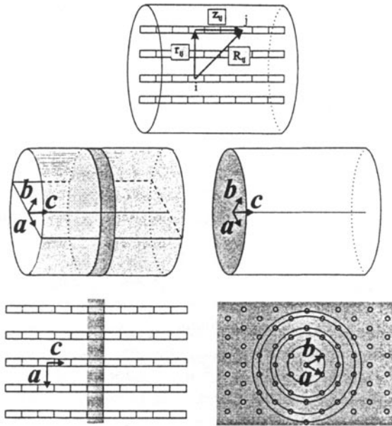
Figure 6. Geometrical arrangement of the antenna. The sites are marked by rectangles. Top: Definition of the distance R_{ij} , r_{ij} and z_{ij} between sites i and j . Left: Cut through the center of the cylindrical microcrystal along a and c . The sites of the shaded area belong to one slab. Right: Cut vertical to c . The channels indicated by circles are arranged in rings around the central channel as a consequence of the hexagonal symmetry 10 .
