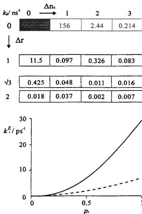
Figure 7. Rate constants for different situations. Top: Energy transfer rate constants k_{ij} in units of 10^9\text{s}^{-1} , for jumps from the shaded site i to neighbour sites j for p_i = 0.25 and J_{ij} = 1.05 \cdot 10^{-13} \text{cm}^3\text{M}^{-1} . Bottom: Depopulation rate constant k_i^E/\text{ps}^{-1} of a site i as a function of the occupation probability p_i for J_{ij} = 4.4 \cdot 10^{-13} \text{cm}^3\text{M}^{-1} (solid) and for J_{ij} = 1.05 \cdot 10^{-13} \text{cm}^3\text{M}^{-1} (dashed).
