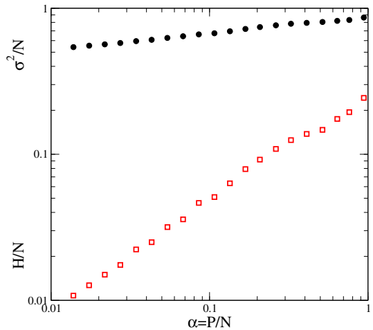
Fig. 6. (Color online) Predictability H/N and fluctuations \sigma^2/N as a function of \alpha = P/N for Poissonian activity ( \theta = 1 ). M = 4 ( P = 16 ), S = 2 , 400NP iterations, 200NP time steps until equilibration, averages over 200 samples.
