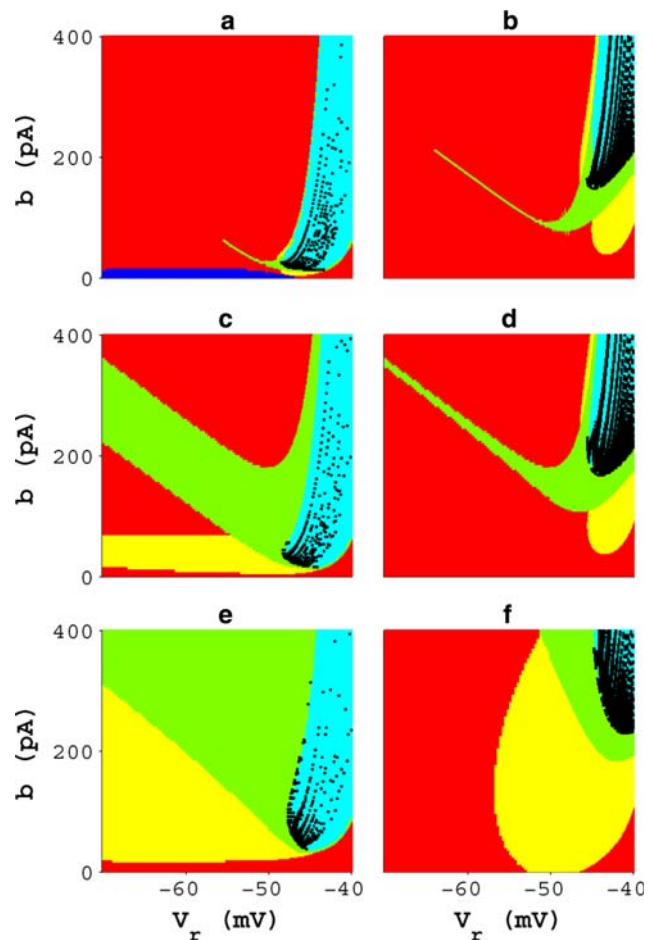
Fig. 6 Parameter space exploration of the four bifurcation parameters. Tonic spiking in red , adapting in yellow , initial bursting in green , regular bursting in cyan , irregular spiking in black and accelerating in blue . The four-dimensional parameter space was reduced to six relevant planes: a adaptive time constant ( \tau_w = 100 ms) and negative a ( a = -5 nS), b refractory time constant ( \tau_w = 5 ms) and negative a ( a = -5 nS), c adaptive time constant ( \tau_w = 100 ms) and low a ( a = 0.001 nS), d refractory time constant ( \tau_w = 5 ms) and low a ( a = 0.001 nS), e adaptive time constant ( \tau_w = 100 ms) and high a ( a = 30 nS), f refractory time constant ( \tau_w = 5 ms) and high a ( a = 30 nS). The firing pattern was classified for injection of current twice the rheobase, according to the criteria exposed in Sect. 3
