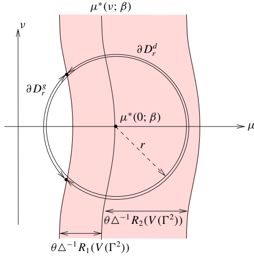
Fig. 2.1. The decomposition of the integral into I_{k,n}^g(\Gamma^2) and I_{k,n}^d(\Gamma^2)
