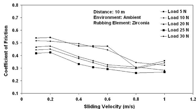
Fig. 3 Variation of coefficient of friction of TiZrNi coatings during sliding against zirconia balls at different normal loads of 5 up to 30 N and sliding velocities of 0.1 up to 1 m/s
