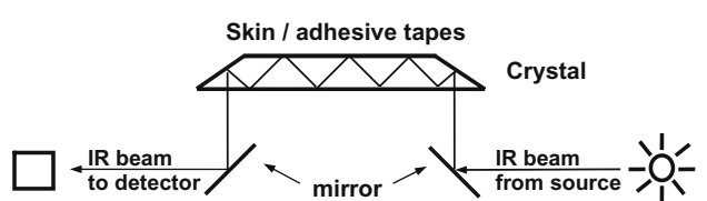
Fig. 7. Schematic diagram of an attenuated total reflectance (ATR) device mounted on a Fourier transform infrared (FTIR) spectrometer. The sampling area of the crystal is made to contact with the treated skin site or the tape-strip. IR radiation from the spectrometer is deflected by a first mirror to the ATR crystal, in which it undergoes total internal reflection, penetrating superficially into the skin, before exiting the crystal and being re-directed to the detector.
