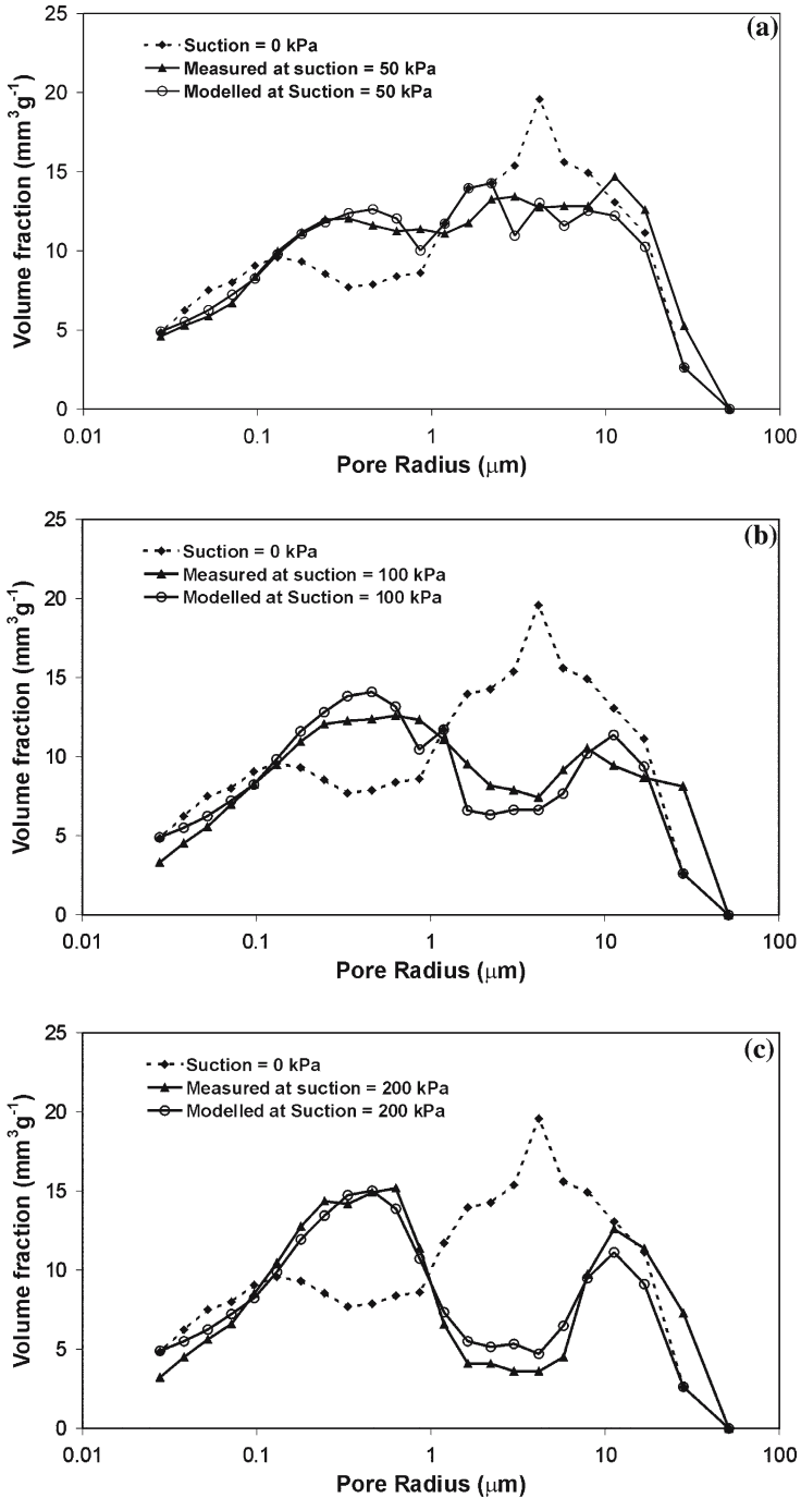
Figure 6. Modelled and measured PSD (a) at suction 50 kPa (b) at suction 100 kPa (c) at suction 200 kPa.
