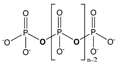
Figure 1. Scheme of a polyphosphate with the chain length n . The oxygen atoms linking two phosphorus atoms together (bold) are called bridging oxygen (BO), while the terminal oxygen atoms in the phosphate groups are called non-bridging oxygen (NBO) [21].
