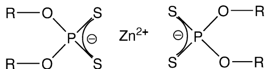
Figure 2. Chemical formula of zinc dialkyldithiophosphate (ZnDTP).
