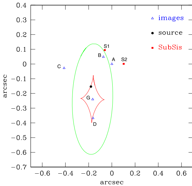
Fig. 3 B1555+375: images, source and galaxy (G) positions are shown assuming a SIE + 2SIS model. The positions of the two substructures are also given. The critical curve and the caustic are for the SIE model alone without the modifications induced by the two substructures
