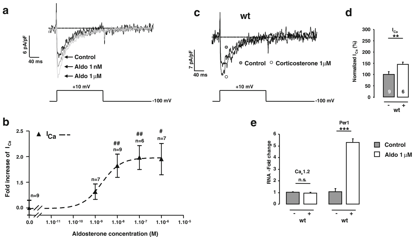
Fig. 2 Concentration–response curves of aldosterone on I_{Ca} of WT cardiomyocytes. a Traces of high-threshold calcium current of control and aldosterone treated (1 nM and 1 μM, 24 h) cardiomyocytes. b Concentration–response curve of aldosterone on I_{Ca} . Data from I_{Ca} (dotted line) was fit according to \% = 1 / (1 + ((\text{drug}) / \text{EC50}))^{100} where EC50 is the drug concentration at half-maximal augmentation; # P < 0.05 , ## P < 0.01 I_{Ca} treated vs untreated. c Representative traces of I_{Ca}
