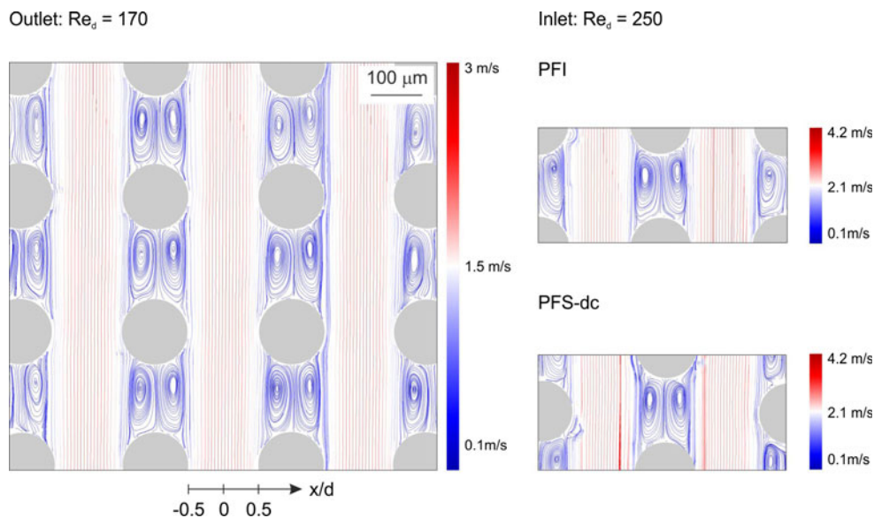
Fig. 5 Ensemble-averaged streamline pattern of the steady flow across the inline pin fin array (final interrogation window 32 \times 32 pixels). For flow rates below the critical Reynolds number, a stable pair of vortices is formed in the space between the pins in the flow direction for both inline and staggered-dc pin arrangement. Whereas the flow at the outlet starts fluctuating at Re_d = 180 , the recirculation zones at the inlet remain stable even at Re_d = 250
