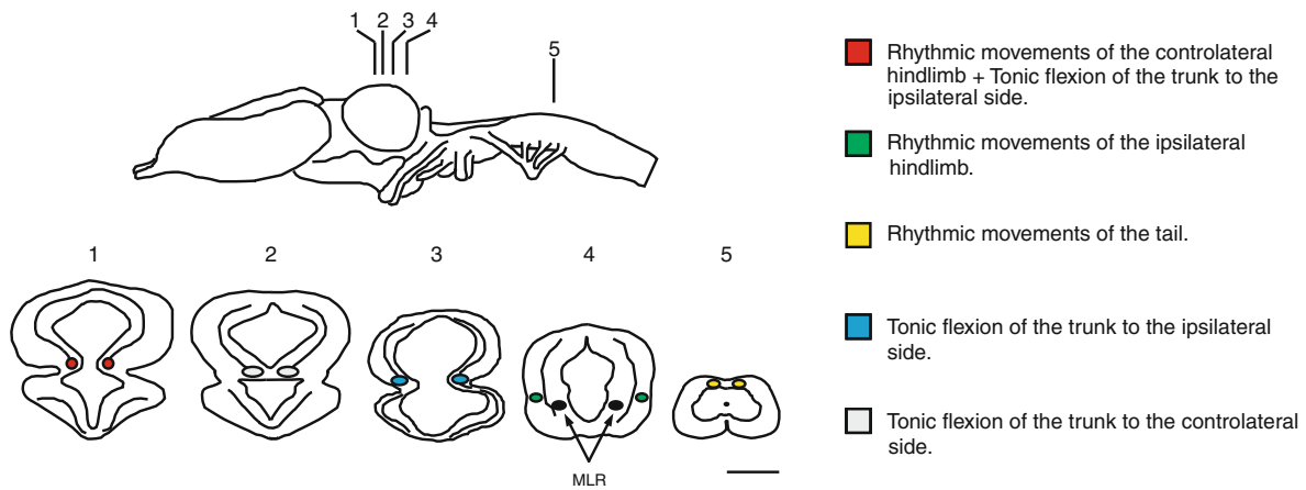
Fig. 4 Stimulation sites that evoked rhythmic and/or tonic movements of different parts of the body in the salamander P. waltlii (stimulation parameters: 2 ms pulses, 2.2–4.8 \mu\text{A} , 10–15 Hz). For comparison the MLR is also indicated. Schematic drawings of transverse sections show
