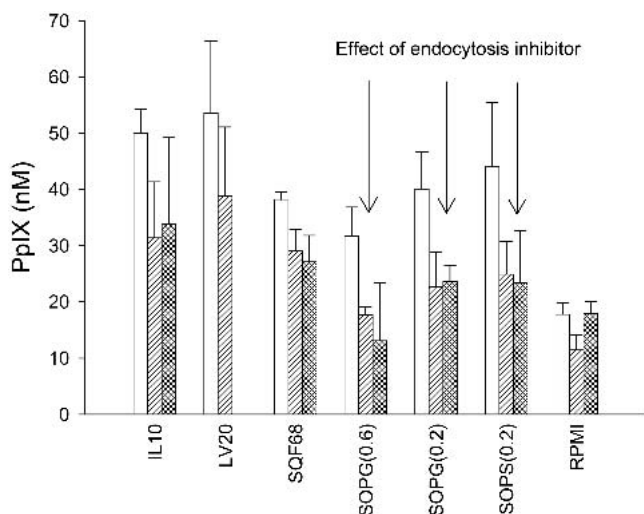
Fig. 5. Inhibition of PpIX production in MCF-7 cells after incubation at 37°C for 1 h with 1 mg/ml ALA in emulsion or RPMI, pH 7.4. No inhibitor (□), 20 mM \text{NH}_4\text{Cl} (▨), 50 mM mannitol (▩). Mean + SD (n = 8).
