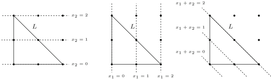
Fig. 5 The max-facet-width of L := \{x \in \mathbb{R}_+^2 : x_1 + x_2 \leq 2\} is w(L) = 2
