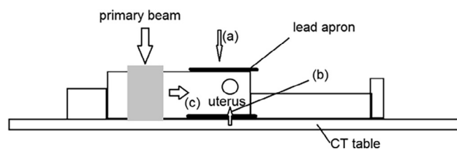
Fig. 1. Schematic depiction of the components of scatter for a chest CT examination using a high Z garment wrapped around the patient's waist. a) External scatter/leakage radiation, b) backscatter from the X-ray table, c) internal scatter.
