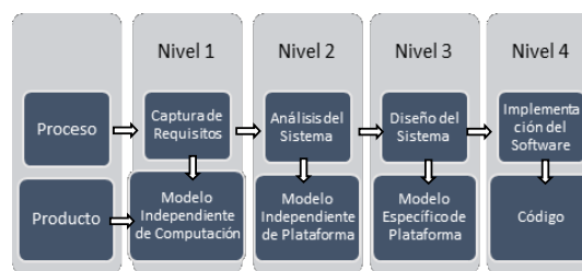
Figura 1. Model-Driven Architecture
