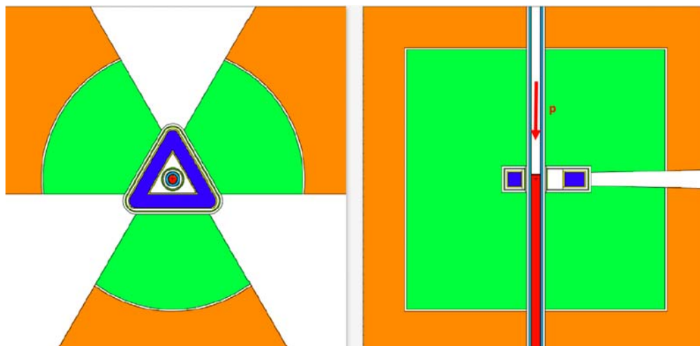
Figure 2. Geometry of the second proposed configuration of compact source using tube moderators. The cold moderator (blue) consists of three tubes filled with parahydrogen, surrounding the Be target (red). The Be reflector is in green, outer steel reflector/shielding in orange. Left: top view (proton beam is perpendicular to the figure), showing neutron beam extraction openings in the reflector. Right: side view, showing proton beam channel, with protons entering vertically from the top.
