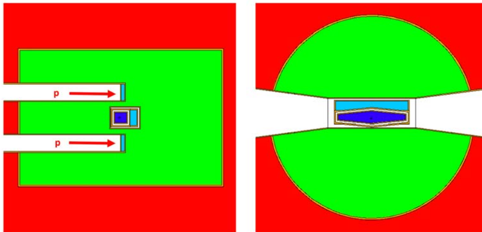
Figure 1. Geometry of the first proposed configuration of compact source using tube moderators [9]. Cold moderator (blue), and thermal moderator (light blue) are surrounded by the Be reflector (green) and outer steel reflector (red). Left: side view showing the two proton beam channels, with proton beams hitting the thin, water-cooled Be targets. Right: top view, showing cold and thermal moderators, with neutron beam extraction channels.
