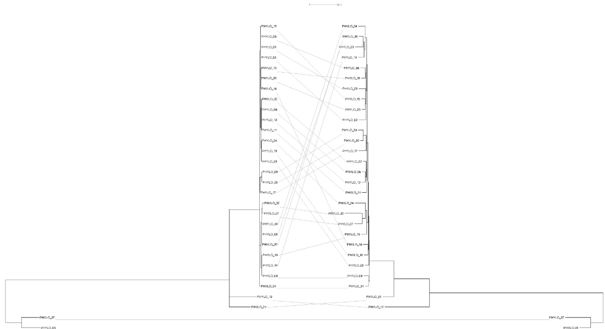
Figure I.2. Tanglegram of the gold standard (left) versus the most different topology produce by Centre 10
