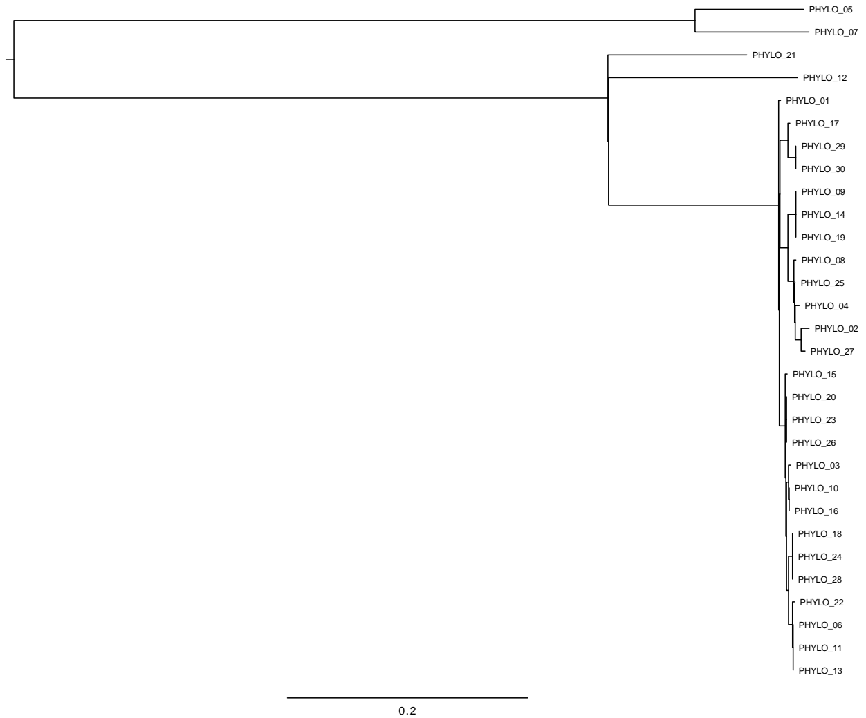
Figure I.8: Phylogeny Centre 4 obtained with CSI Phylogeny (CGE tools, online version)
