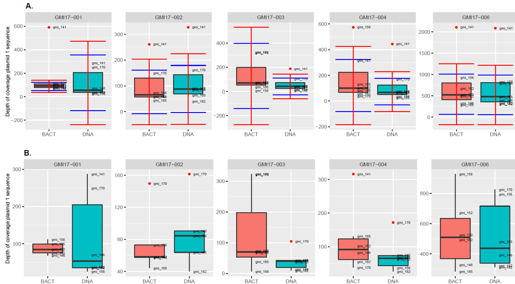
Figure M.17: Depth of coverage, plasmid 1 sequence
