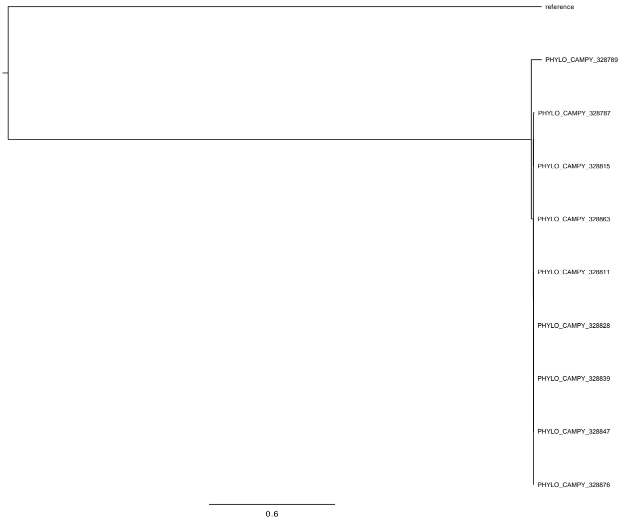
Figure J.13: Phylogeny results Centre 8
