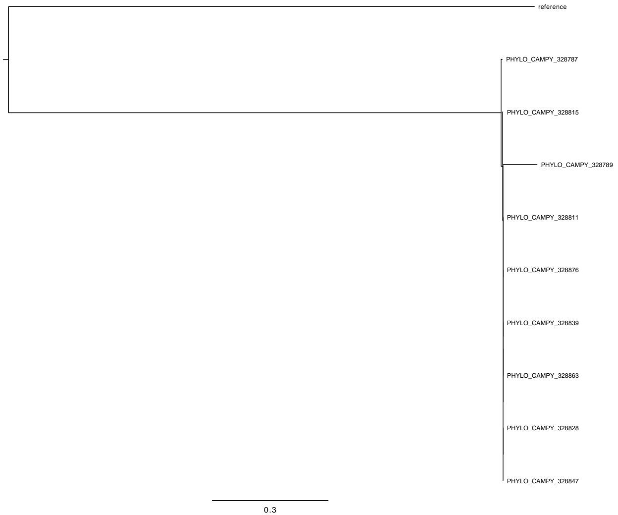
Figure J.11: Phylogeny results Centre 6
