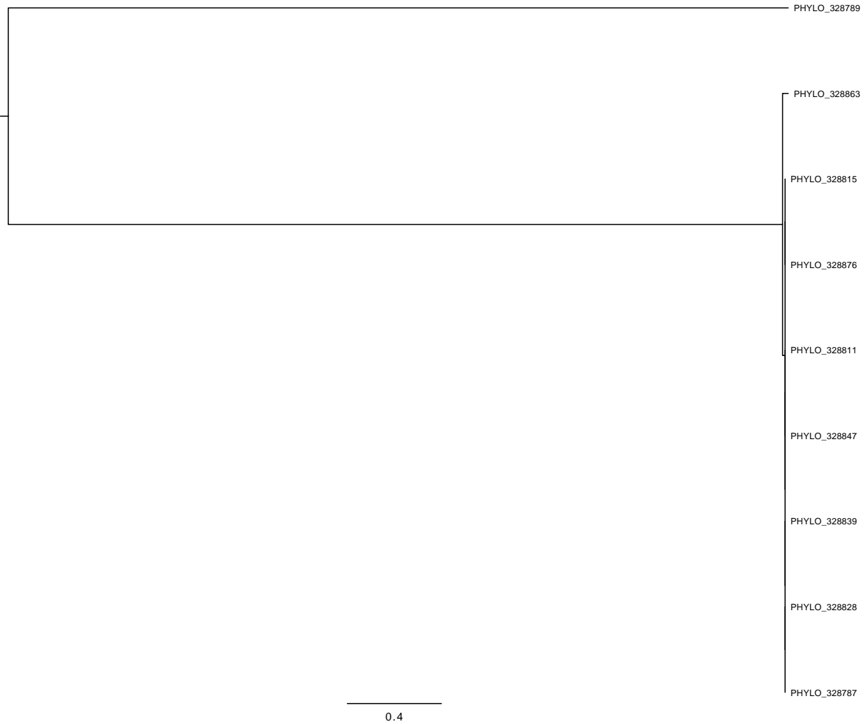
Figure J.16: Phylogeny results Centre 11
