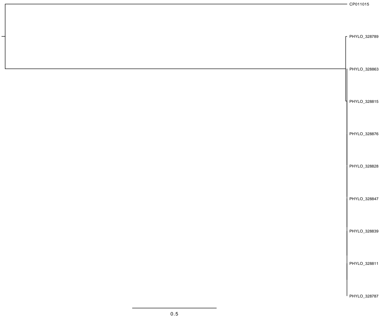
Figure J.15: Phylogeny results Centre 10
