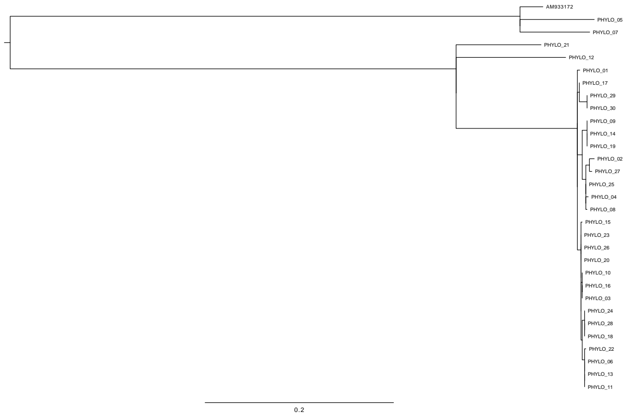
Figure I.15: Phylogeny Centre 11 obtained with PHENix/SnapperDB and for variants detection and RAxML for tree building
