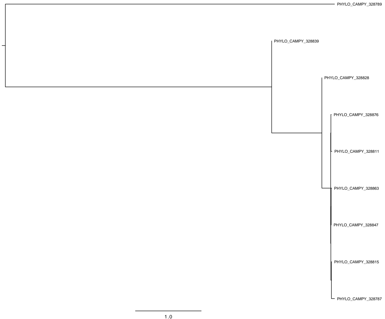
Figure J.14: Phylogeny results Centre 9
