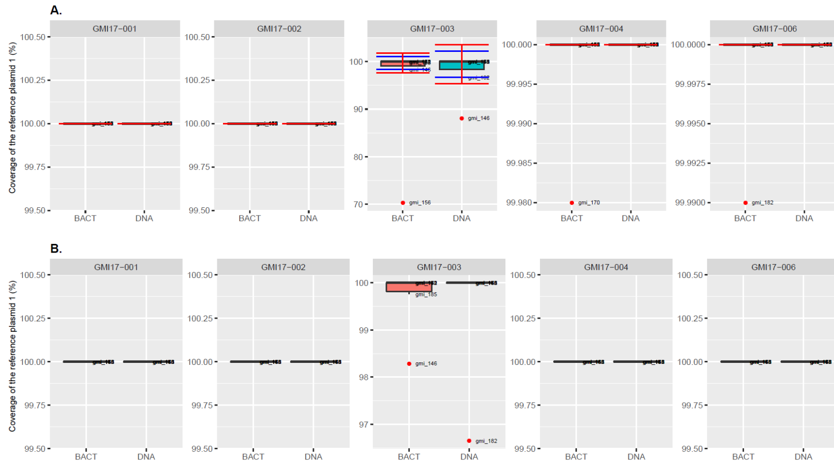
Figure M.22: Coverage of reference plasmid 1
