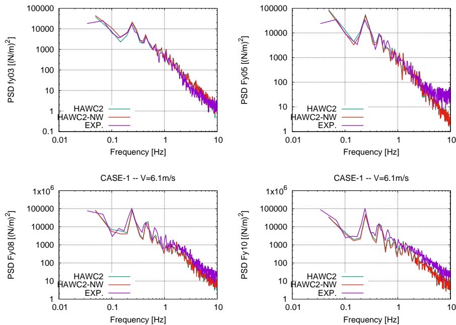
Figure 6: Spectra of the normal to chord force component simulated with the HAWC2 and HAWC2-NW code, respectively, in comparison with spectra of the measured forces.
