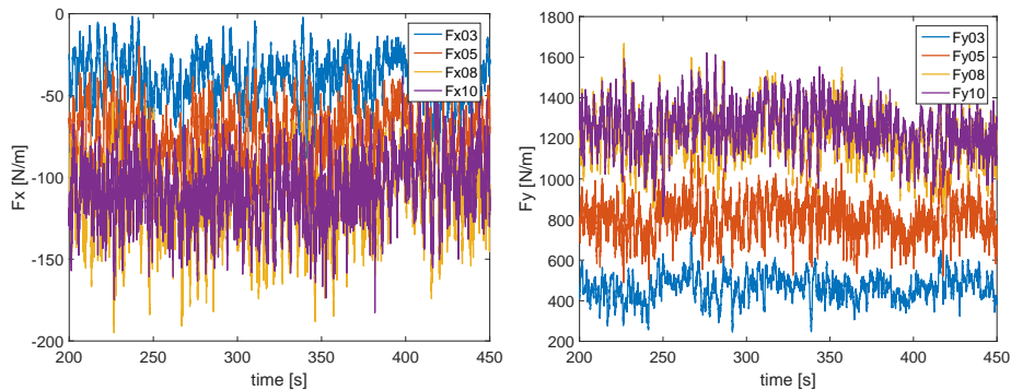
Figure 3: The aerodynamic sectional forces f_x , f_y in direction chordwise and perpendicular to the chord, respectively, integrated from the measured pressure distributions.
