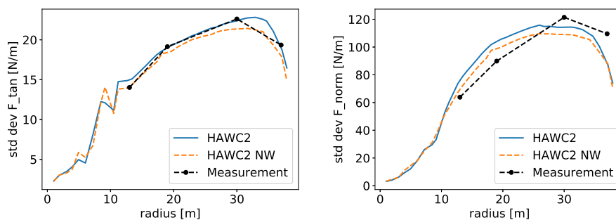
Figure 7: Std. dev. along the blade span of the unsteady aerodynamic force component tangential and normal to the chord, respectively, simulated with the HAWC2 and HAWC2-NW code and measured ones.
