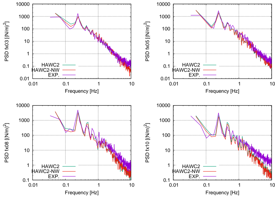
Figure 5: Spectra of the chordwise force component simulated with the HAWC2 and HAWC2-NW code, respectively, in comparison with spectra of the measured forces.
