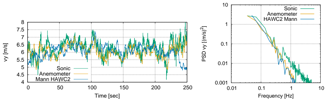
Figure 4: The wind speed variation and the PSD of the velocity component in the flow direction in the center of the Mann box in comparison with time variation and PSD of the hub height anemometer and sonic measurement.
