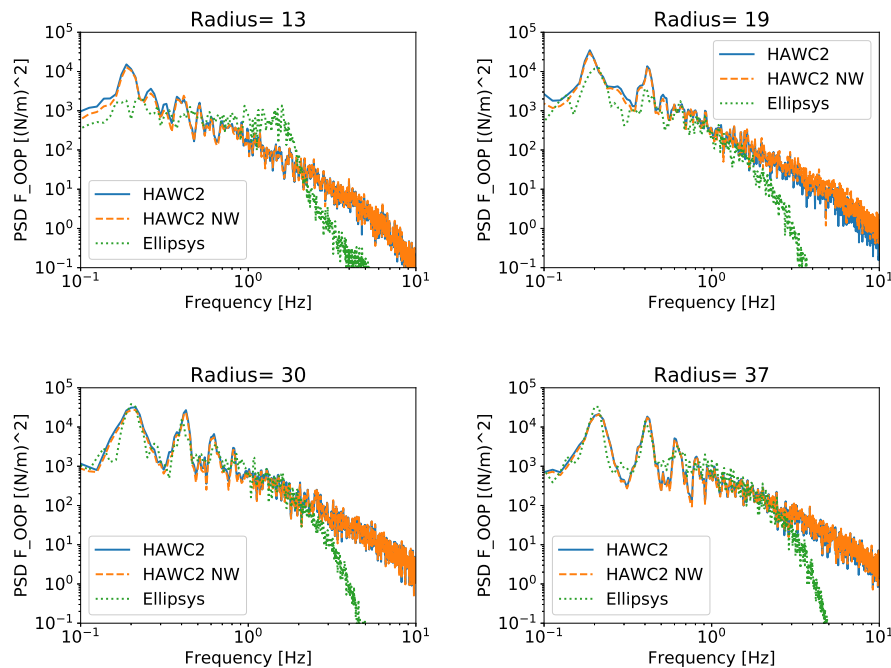
Figure 10: Spectra of the out of plane force component simulated with the EllipSys3D code in comparison with HAWC2 and HAWC2-NW simulations.
