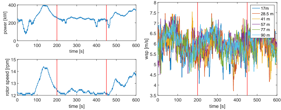
Figure 2: The 250 sec data set was chosen because as seen in the left figure, indicated between the red lines, the rotor speed is almost constant and close to 12 rpm. In the right figure the wind speed at six heights measured in the nearby meteorology mast indicate that the wind shear is low.
