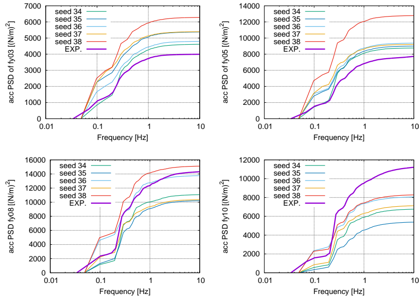
Figure 8: Accumulated spectra of the normal to chord force component simulated with the HAWC2 code for different seed numbers in the turbulence generation and compared with accumulated spectra of the measured forces.
