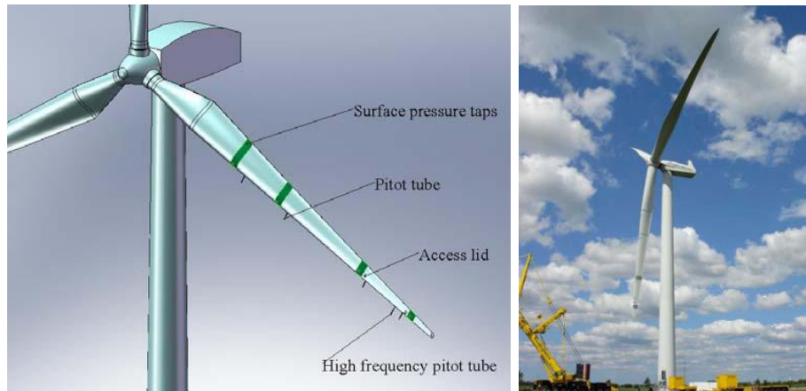
Figure 1: Left: Sketch showing an overview of the instrumentation of the test blade. Right: The test blade after installation on the turbine in May 2009, replacing one of the original blades.
