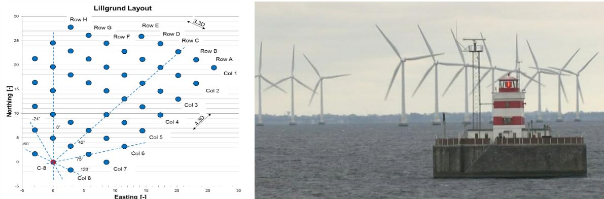
Figure 2. Layout of the Lillgrunden WF with the instrumented WT C-8 marked. Distances are non-dimensional with the rotor diameter. Also shown is Drogden light tower located WNW of the WF. The distance between WF and the light tower roughly corresponds to a characteristic scale of the WF.
