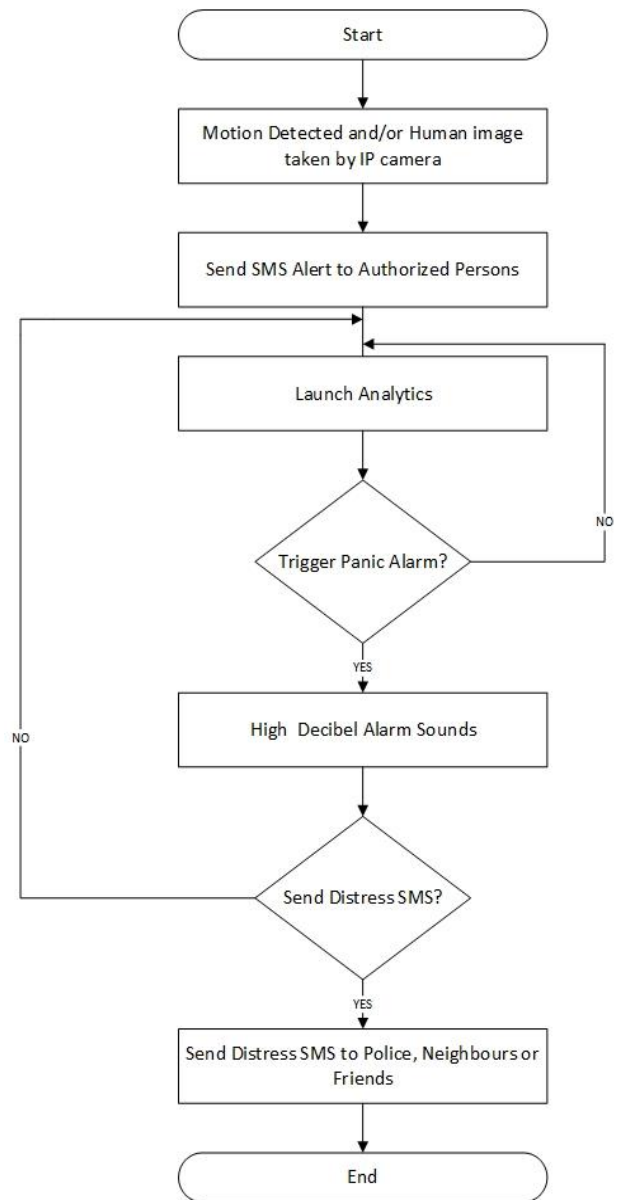
Figure 3 : Flowchart of Implemented Analytics Based Anti-Intruder Monitoring and Alarm System.
