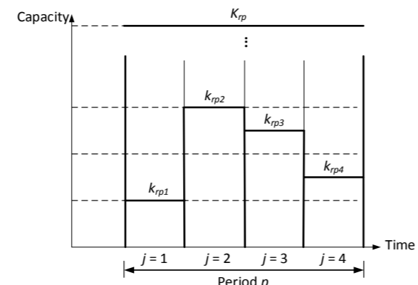
FIGURE 01. Illustration of disaggregating resource capacities
