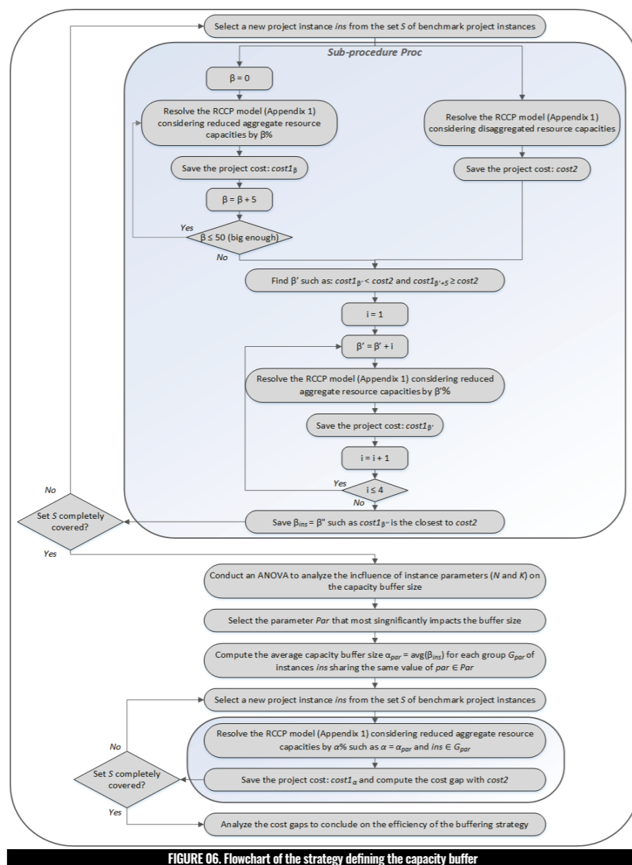
FIGURE 06. Flowchart of the strategy defining the capacity buffer
