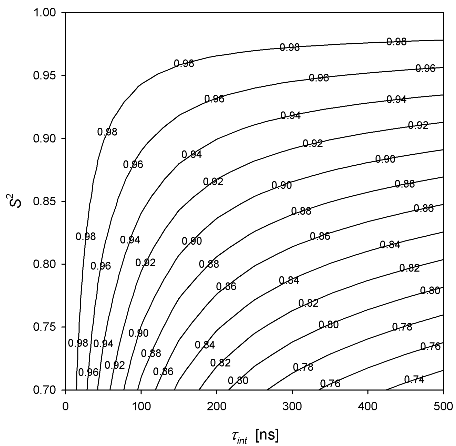
Figure S1 Contour plot presenting Q values normalized in relation to the Q in rigid molecule. \tau_R=10 ns and B_0=14.1 T were used in calculations.
