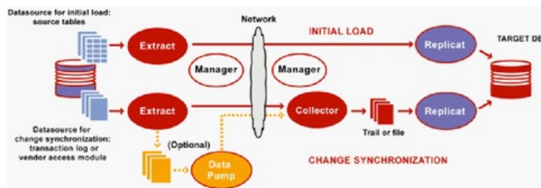
Fig. 2: Components of Oracle Golden Gate
