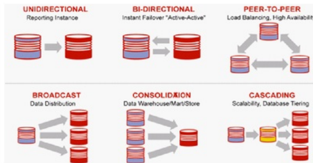
Fig. 1: Supported topologies by Oracle Golden Gate
