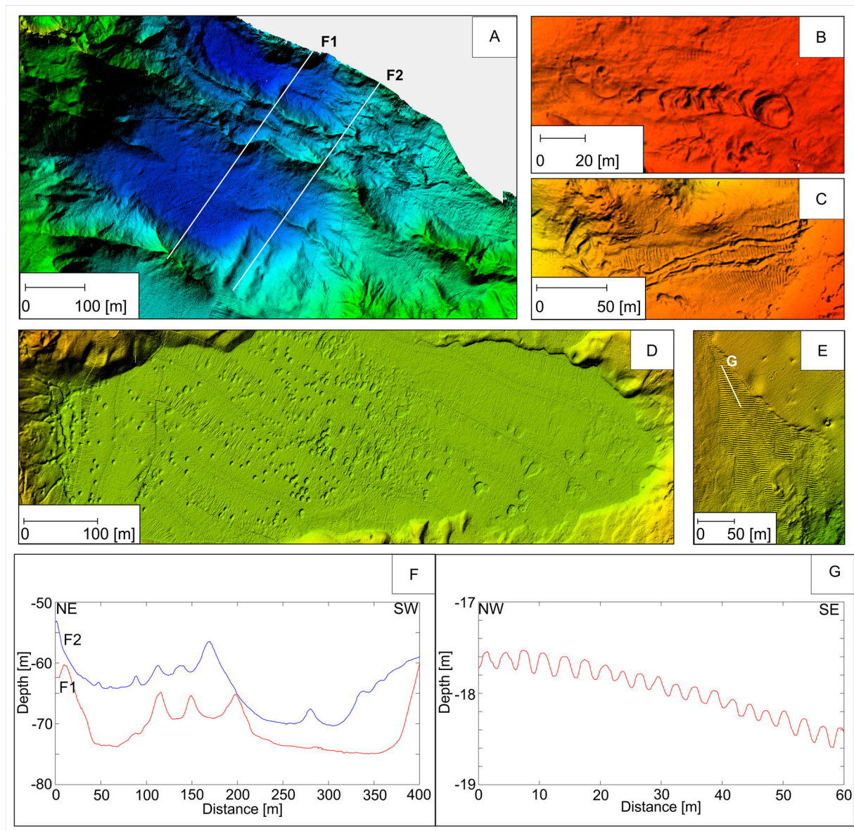
Figure 5. Details of selected morphological features. For the location, see Figure 1. (A) Moderate-size moraine ridges with adjacent flat-floored areas; (B) Example of a chain of iceberg-generated pits; (C) Iceberg-generated ploughmarks; (D) Pockmarks on the flat-floored area; (E) Field of megaripples, (F) Morphological profiles across moderate-size moraines (marked on Figure 5(A)); (G) Profile across the field of megaripples (marked on (E)).
