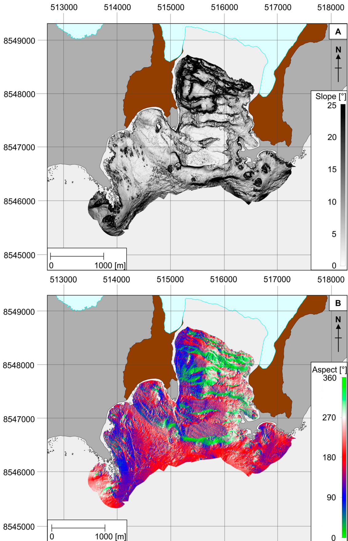
Figure 3. Slope characteristics in Isbjørnhamna and Hansbukta. (A) Slope inclination; (B) slope aspect.
