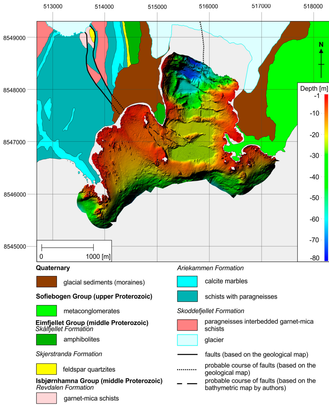
Figure 2. Bedrock and Quaternary geology around Isbjørnhamna and Hansbukta (after Birkenmajer, 1990; Czerny et al., 1993 and Majka, Czerny, Mazur, Holm, & Manecki, 2010). Bathymetry after the Main Map.
