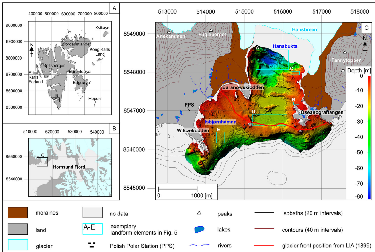
Figure 1. Study area. (A) Location of the study area within Svalbard; (B) – Study area within Hornsund Fjord; (C) Isbjørnhamna and Hansbukta bathymetry after the Main Map. The boxes named 'a' to 'e' refer to the locations of the landforms presented in detail in Figure 5. Sources: Norwegian Polar Institute: http://geodata.npolar.no/ and swath bathymetry data from Norwegian Hydrographic Service (permit no. for IG PAS: 13/G722).
