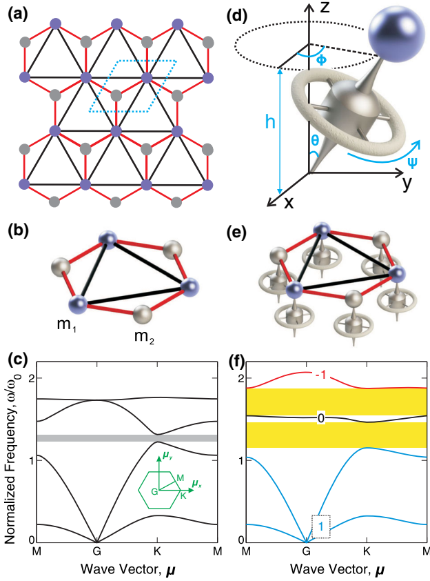
FIG. 1 (color online). Ordinary and gyroscopic phononic crystals: (a) Schematic of the hexagonal lattice. The blue and grey spheres represent concentrated masses m_1 and m_2 = m_1 , respectively. The red and black straight rods represent massless linear springs with stiffness k_1 and k_2 = k_1/20 , respectively. The dashed cell is the primitive cell of the lattice. (b) Unit cell for the ordinary (nongyroscopic) phononic crystal. (c) Band structure of the ordinary (nongyroscopic) phononic crystal. The inset is the Brillouin zone. (d) Schematic of a gyroscope with the top tip pinned to a mass in the lattice. (e) Unit cell for the gyroscopic phononic crystal. (f) Band structure of the gyroscopic phononic crystal ( \alpha_1 = \alpha_2 = 0.3m_1 ) with the Chern numbers labeled on the bulk bands. The frequencies are normalized by \omega_0 = \sqrt{k_1/m_1} .
