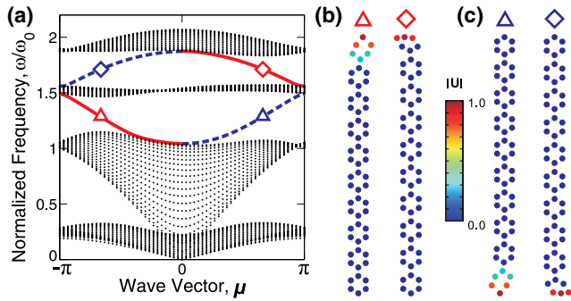
FIG. 2 (color online). Edge modes in gyroscopic phononic crystal: (a) 1D band structure showing bulk bands (black dots) and edge bands (colored lines). Red solid lines represent edge modes bound to the top boundary, while blue dashed lines represent edge modes bound to the bottom boundary. (b) Modal displacement fields of top edge states with negative group velocities. (c) Modal displacement fields of bottom edge states with positive group velocities.
