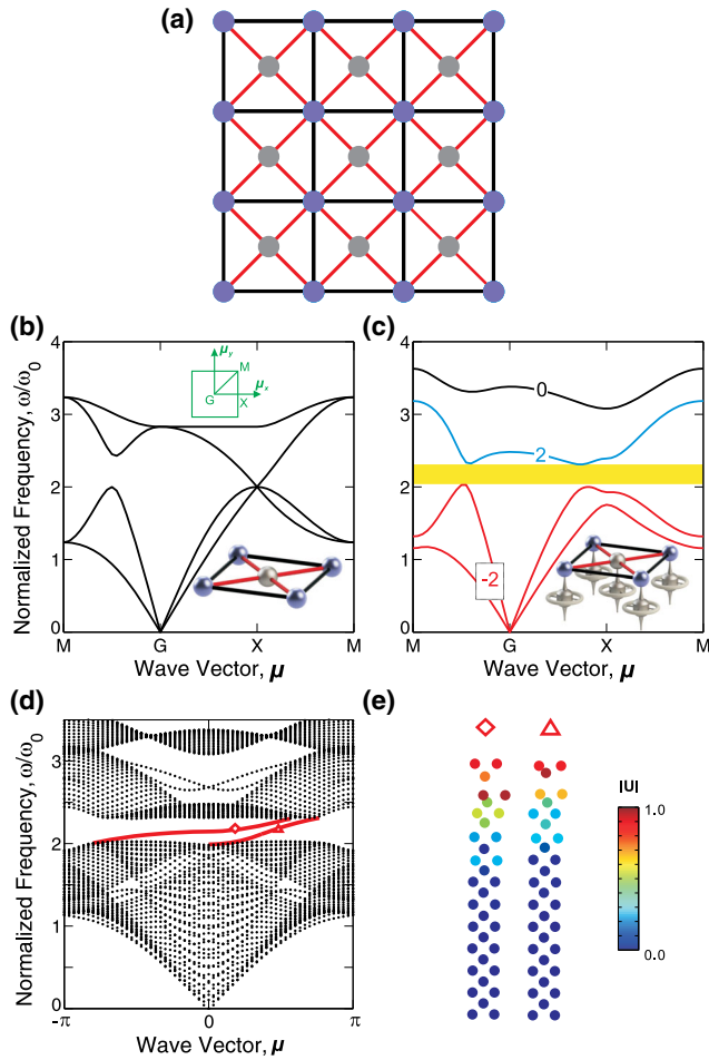
FIG. 4 (color online). Square lattice results: (a) Schematic of the square lattice. The blue and grey spheres represent concentrated masses m_1 and m_2 = m_1 , respectively. The black and red straight rods represent massless linear springs with stiffness k_1 and k_2 = 2k_1 , respectively. (b) Band structure of the ordinary (nongyrosopic) phononic crystal. The insets are the Brillouin zone and the unit cell. (c) Band structure of the gyrosopic phononic crystal ( \alpha_1 = \alpha_2 = 0.3m_1 ) with the Chern numbers labeled on the bulk bands. Frequencies are normalized by \omega_0 = \sqrt{k_1/m_1} . The inset is the unit cell. (d) 1D band structure showing bulk bands (black dots) and two topological edge bands (red solid lines) bound to the top boundary. Note that the edge bands that are bound to the bottom boundary are not shown here. (e) Modal displacement fields of the edge states shown in (d).
