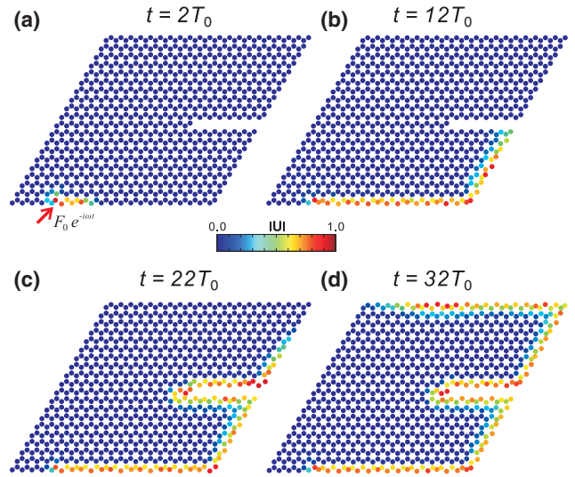
FIG. 3 (color online). Transient response of a gyroscopic phononic crystal consisting of 20 \times 20 unit cells with a line defect on the right boundary: Snapshots of the displacement field at (a) t = 2T_0 , (b) t = 12T_0 , (c) t = 22T_0 and (d) t = 32T_0 , where T_0 = \sqrt{m_1/k_1} is the characteristic time scale of the system. Starting from t = 0 , a time-harmonic excitation force \mathbf{F}(t) = [F_x(t), F_y(t)] = [1, 1]F_0 e^{-i\omega t} is prescribed at the site indicated by the red arrow.
