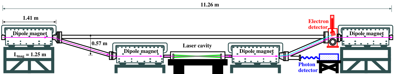
Fig. 2. Schematic of the JLab Hall-C Compton polarimeter. Figure taken from [6].
