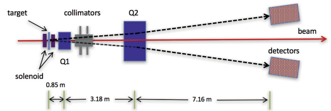
Fig. 1. Schematic of the JLab Hall-C Møller polarimeter. Note that the quadrupole positions are slightly different than described in Ref. [8].
