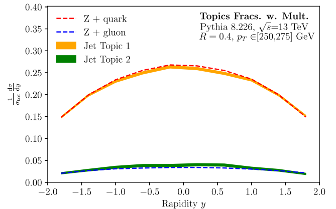
FIG. 3. Cross sections for jet topics (orange and green) using topic fractions extracted from the Z + \text{jet} sample across ten rapidity bins. The extracted topic cross sections closely track the underlying Z + \text{quark} and Z + \text{gluon} cross sections (red and blue).
