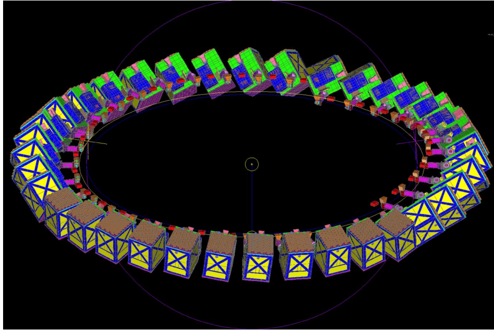
Figure 8. Solar illumination simulation for a representative sequence of three target observations with NICER for an ISS orbit beta angle of +25^\circ . The view is from the Sun, with orbit noon at bottom and the sequence progressing counterclockwise.
