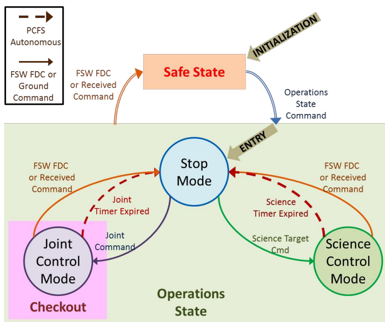
Figure 7. Pointing Control Flight Software mode transition diagram.
