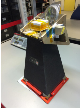
Figure 5. NICER's \mu ASC star tracker, developed by the Technical University of Denmark. The camera head and baffles are shown mounted on an IOB bracket.
