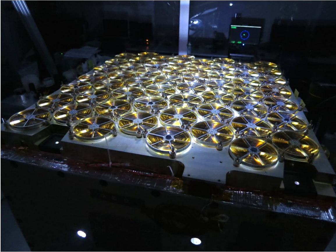
Figure 3. NICER's 56 X-ray Concentrator optics integrated onto the Concentrator Plate in NICER's dedicated coalignment facility.
