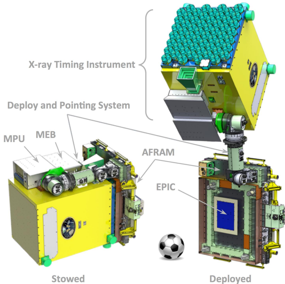
Figure 1. NICER in its stowed and deployed configurations.
