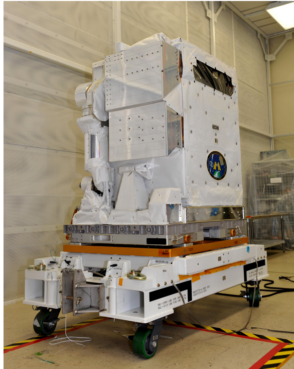
Figure 2. The NICER flight payload in a nearly fully integrated configuration, blanketed and stowed against the flight A-FRAM plate.
