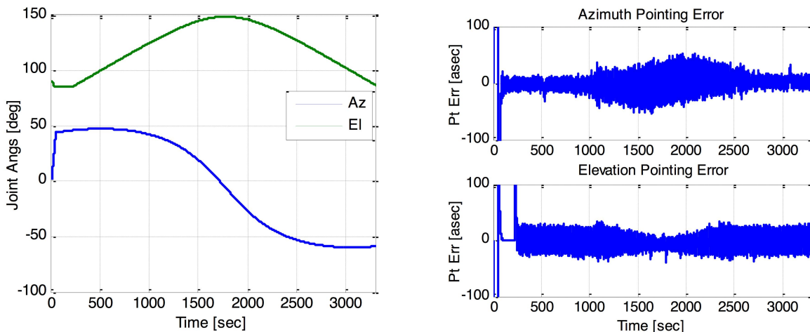
Figure 6. Joint angles ( left ) and pointing error ( right ) from the high-fidelity NICER pointing simulation.
