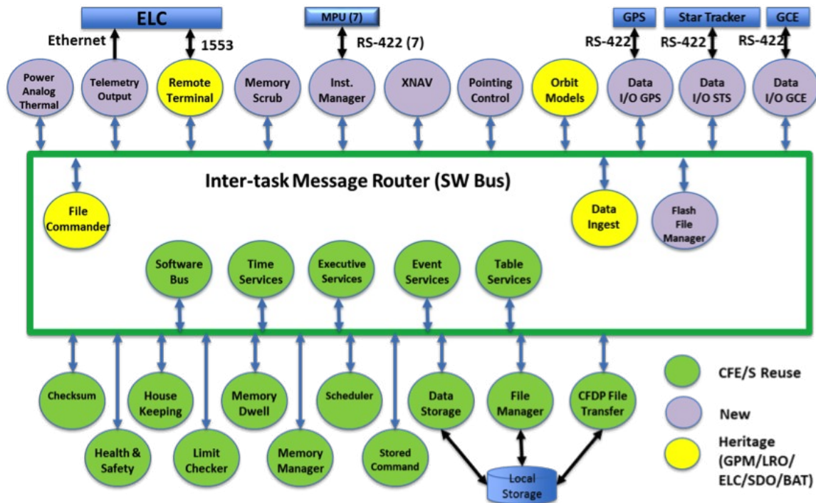
Figure 9. NICER flight software architecture.
