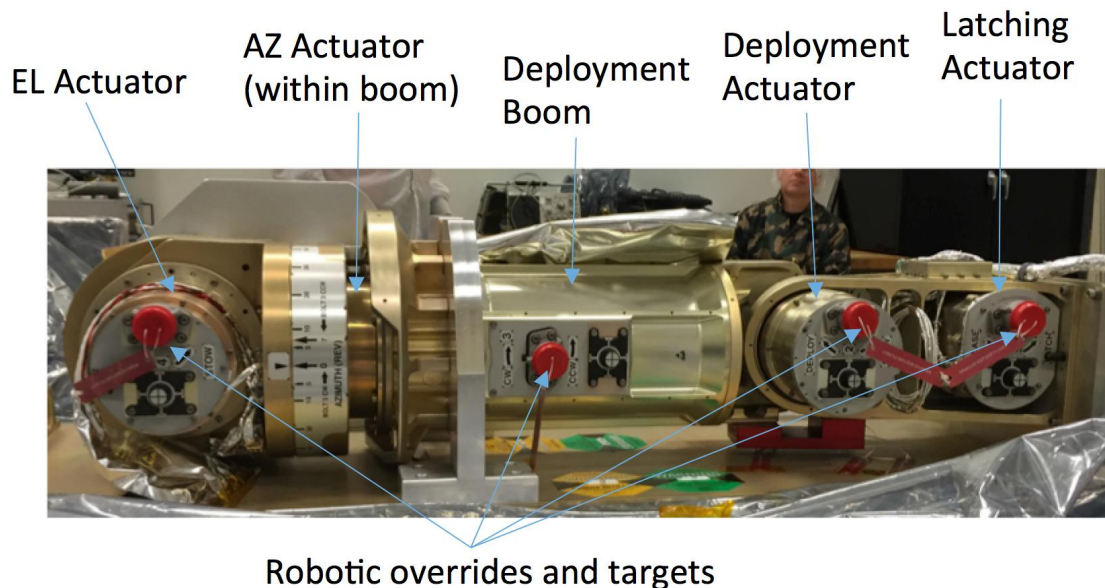
Figure 4. DAPS mechanism assembly, developed by Moog Chatsworth, Inc.
