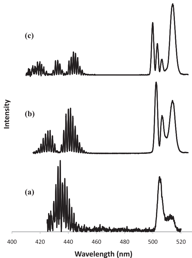
FIG. 3. Experimental NaCs 12(0^+) \rightarrow 1(X)^1\Sigma^+ bound-bound and 12(0^+) \rightarrow 1(a)^3\Sigma^+ bound-free resolved fluorescence spectra associated with the three lowest vibrational levels of the NaCs 12(0^+) state. Upper state vibrational and rotational quantum numbers are (a) (0, 43), (b) (1, 43), and (c) (2, 43). Vibrational quantum number assignments are explained in Sec. IV. The 12(0^+) \rightarrow 1(X)^1\Sigma^+ bound-bound fluorescence appears as a series of discrete vibrational peaks in the 410–460 nm region, while the 12(0^+) \rightarrow 1(a)^3\Sigma^+ bound-free continuum fluorescence is observed in the 500–520 nm region. Each spectrum has been corrected for the wavelength dependence of the detection system efficiency, resulting in an increase in the apparent noise level at the short wavelength end of each spectrum.
