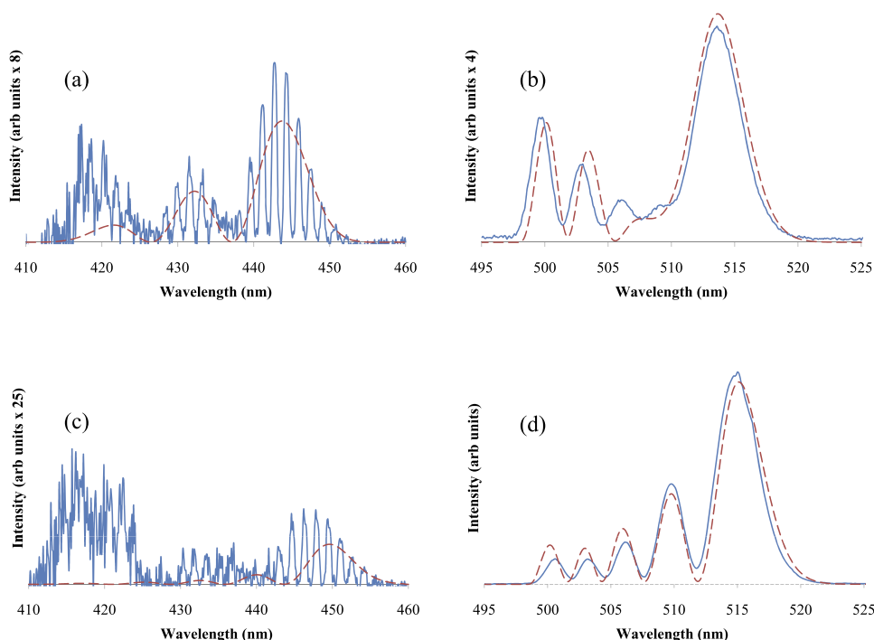
FIG. 8. Comparison of experimental (solid—blue) and simulated (dashed—red) spectra for (a) 12(0^+) (2, 33) \rightarrow 1(X)^1\Sigma^+ , (b) 12(0^+) (2, 33) \rightarrow 1(a)^3\Sigma^+ , (c) 11(0^+) (4, 33) \rightarrow 1(X)^1\Sigma^+ , and (d) 11(0^+) (4, 33) \rightarrow 1(a)^3\Sigma^+ transitions. The intensity distributions result from mixing pure 11(0^+) (4, 33) and 12(0^+) (2, 33) vibrational wavefunctions according to Eqs. (23) and (24) with (b_1/a_1) = -0.0472 \pm 0.0001 , (a_2/b_2) = 0.2878 \pm 0.0001 , and \theta = 0.328 \pm 0.003 radians.
