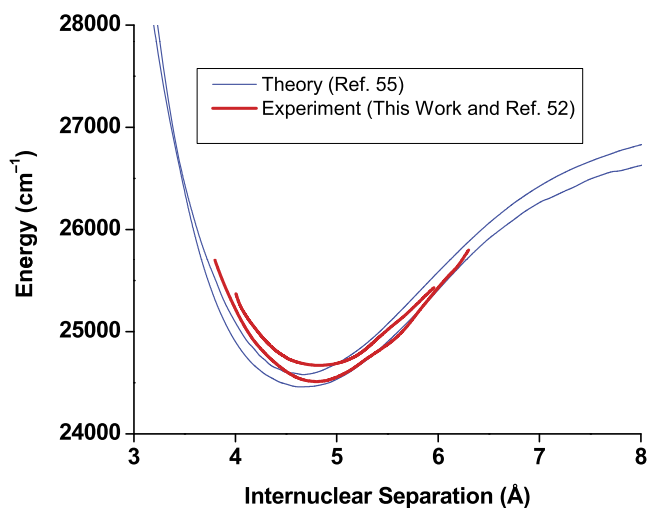
FIG. 4. Experimental IPA potential for the NaCs 12(0^+) state determined in this work along with the experimental potential for the NaCs 11(0^+) state from Ref. 52 (upper and lower thick red lines, respectively) and the NaCs 12(0^+) and 11(0^+) theoretical potentials of Korek et al. 55 (upper and lower thin blue curves, respectively). The Korek et al. ground state well depth is larger by 298.214 \text{ cm}^{-1} than the experimental ground state well depth of Ref. 44. Since the T_e values reported in Ref. 55 are based on energies relative to the bottom of this theoretical ground state potential, while our experimental 11(0^+) and 12(0^+) potentials are referenced to the bottom of the experimental ground state potential of Ref. 44, we have shifted the theoretical curves down by 298.214 \text{ cm}^{-1} so that the ground state asymptotes of the theoretical and experimental potentials coincide. We believe this makes the comparison of the theoretical and experimental potentials more meaningful.
