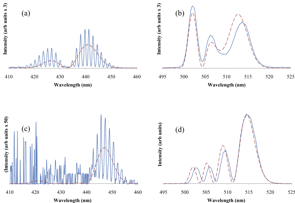
FIG. 7. Comparison of experimental (solid—blue) and simulated (dashed—red) spectra for (a) 12(0^+) (1, 43) \rightarrow 1(X)^1\Sigma^+ , (b) 12(0^+) (1, 43) \rightarrow 1(a)^3\Sigma^+ , (c) 11(0^+) (3, 43) \rightarrow 1(X)^1\Sigma^+ , and (d) 11(0^+) (3, 43) \rightarrow 1(a)^3\Sigma^+ transitions. The intensity distributions result from mixing pure 11(0^+) (3, 43) and 12(0^+) (1, 43) vibrational wavefunctions according to Eqs. (23) and (24) with (b_1/a_1) = -0.195 \pm 0.001 , (a_2/b_2) = 0.2116 \pm 0.0001 , and \theta = 0.311 \pm 0.002 radians.
