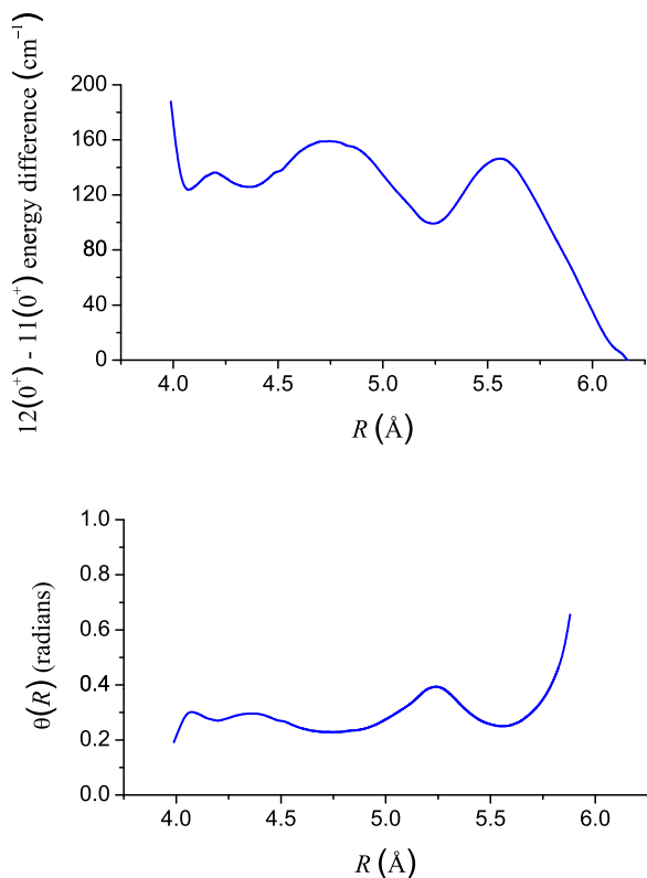
FIG. 9. (a) Difference in energy of the NaCs 12(0^+) and 11(0^+) experimental electronic potentials (from this work and Ref. 52, respectively), as a function of internuclear separation R . (b) Mixing angle \theta(R) describing the spin-orbit interaction between the 7^1\Sigma^+ and 5^3\Pi_0^+ electronic states [see Eq. (29)].
