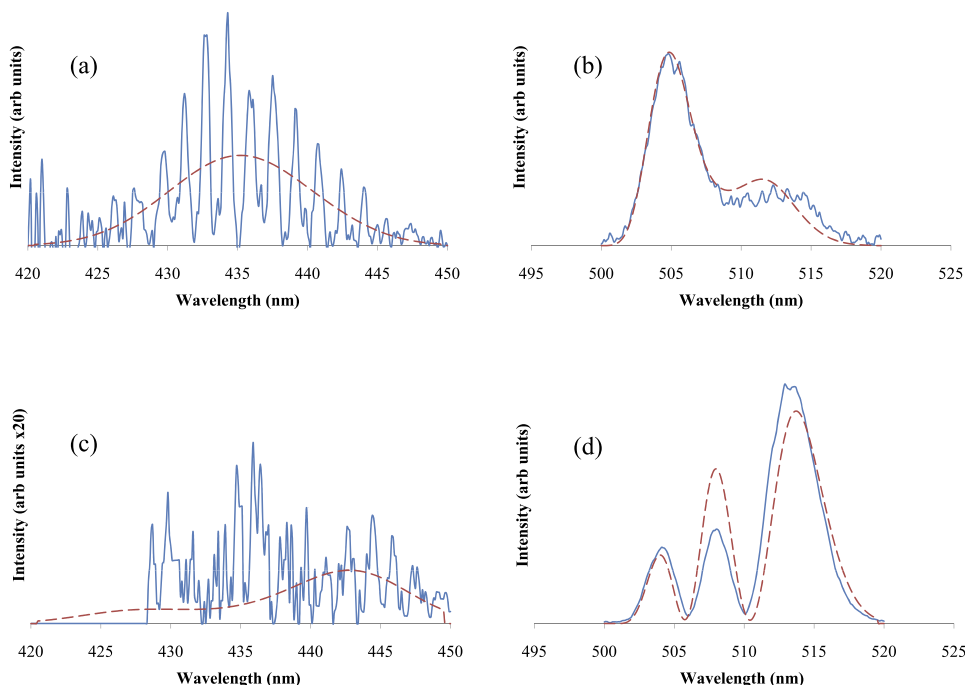
FIG. 6. Comparison of experimental (solid—blue) and simulated (dashed—red) spectra for (a) 12(0^+) (0, 43) \rightarrow 1(X)^1\Sigma^+ , (b) 12(0^+) (0, 43) \rightarrow 1(a)^3\Sigma^+ , (c) 11(0^+) (2, 43) \rightarrow 1(X)^1\Sigma^+ , and (d) 11(0^+) (2, 43) \rightarrow 1(a)^3\Sigma^+ transitions. The intensity distributions result from mixing pure 11(0^+) (2, 43) and 12(0^+) (0, 43) vibrational wavefunctions according to Eqs. (23) and (24) with (b_1/a_1) = -0.486 \pm 0.002 , (a_2/b_2) = 0.1032 \pm 0.0008 , and \theta = 0.248 \pm 0.007 radians.
