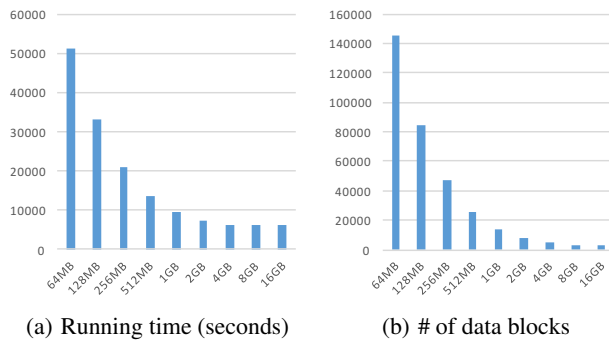
Figure 14: Effect of varying size of memory buffer
