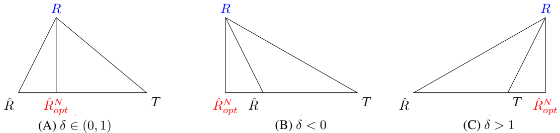
Diagram 1: Geometric illustration of shrinkage estimators. R is the truth, T is the target, \hat{R} is the sample correlation, \hat{R}_{opt}^N is the “oracle” NOVELIST estimator defined as the linear combination of T and \hat{R} with minimum spectral norm distance to R . LEFT: \delta \in (0, 1) if target T is appropriate; MIDDLE: \delta < 0 if target T is misspecified; RIGHT: \delta > 1 if \hat{R} is far from R .
