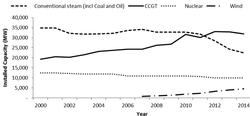
Fig. 1. BETTA installed capacity [5].
