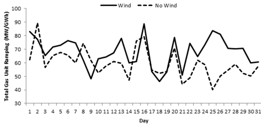
Fig. 3. Change in gas unit ramping due to wind power [89].
