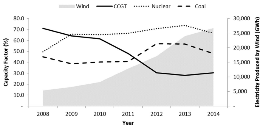
Fig. 2. BETTA generation capacity factor v wind generation [5].
