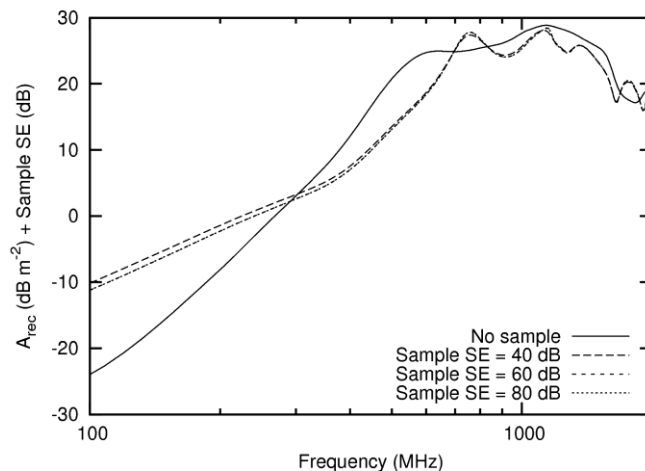
Figure 7. Results of the TLM model comparing the reception aperture normalised by the known SE of the numerical sample for different sample characteristics. Note that the curves for T=-60 dB and T=-80 dB overlay.
