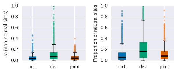
Figure 2. Estimates of sequence evolution in a nearly neutral model. Distributions of \omega = d_N/d_S values (left panel) and the proportion of the neutrally evolved sites (right panel) for ordered (blue), disordered (green), and ordered and disordered protein regions jointly analyzed (orange).
