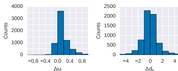
Figure 1. Histograms of paired differences in \omega ( \omega = d_N/d_S ) and d_S values in proteins with disordered and ordered protein regions. Shown are the pairwise differences in disordered minus ordered protein regions ( \Delta\omega and \Delta d_S ) of the same protein. Substitution rates for nonsynonymous ( d_N ) and synonymous ( d_S ) sites are obtained from a one-ratio model. \omega values are significantly different for ordered and disordered regions (Wilcoxon signed-rank test, paired, P < 2.2 \times 10^{-16} ); the difference d_S has a greater P -value ( P < 4 \times 10^{-4} ).
