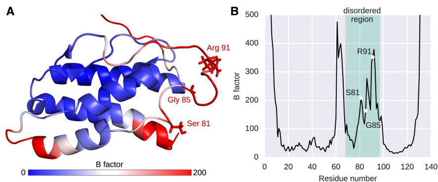
Figure 3. Three-dimensional features of positively selected sites in the disordered region of human interleukin 21. (A) Cartoon of the NMR structure of human interleukin 21 (PDB Code: 2OQP) including its disordered region indicating B-factor scores from the molecular dynamics analysis. Three residues have been identified as positively selected in a PAML branch-site test (Ser81, Gly85, and Arg91) in the disordered region. (B) Molecular dynamics analysis; shown are the B-factors of all residues. Here, B-factors reflect the fluctuation of single amino acids ( C_{\alpha} atom) about their average positions during the MD simulation. The predicted disordered region by MobiDB is indicated in green as well as the three identified residues under positive selection (S81, G85, and R91).
