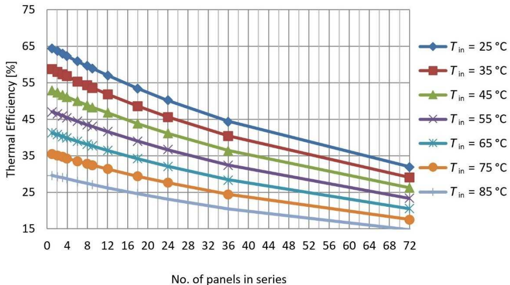
Figure 15. PVT thermal efficiency for different inlet temperature
