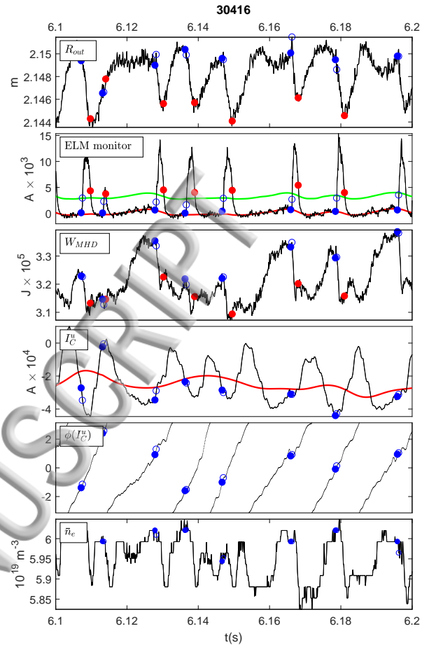
FIG. 4: Time traces plotted for a 0.1 s time window (of the same duration as in Fig. 1) at a time before the transition to synchronous dynamics in plasma 30416. Format is as in Fig.1. This short time interval is indicated by the blue bar in Figure 3 top panel.
