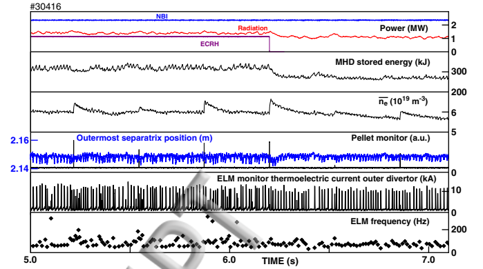
FIG. 2: Experimental plasma parameters for the latter part of plasma 30416. Top panel: Neutral beam injection (NBI) heating (blue line) and plasma radiation (red line) are constant. Electron cyclotron resonant heating (ECRH, purple line) is stepped down at t = 6.2s . Second panel: Total MHD stored energy which drops at ECRH switch-off. Third panel: Line averaged plasma density which is enhanced on pellet injection. Fourth panel: Pellet monitor spikes identify pellet times. Fifth panel: ELM monitor (blue line) from which we identify the ELM occurrence times as the rise in the thermoelectric current observed at a tile in the divertor region, and pellet monitor (black line) and sixth panel: ELM frequency.
