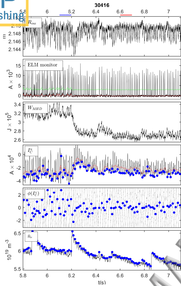
FIG. 3: Vertical control system current temporal phase just before each natural ELM becomes localised following the transition to synchronous dynamics which occurs after t \simeq 6.2 s in plasma 30416. The format of the plot is a simplified version of that of Fig. 1. from top to bottom (black traces): the edge position ( R_{out} ); the ELM monitor; the total plasma MHD energy ( W_{MHD} ); the current in the upper vertical control system coil ( I_C^u ); its analytic temporal phase ( \phi(I_C^u) ) and the averaged plasma density ( \bar{n}_e ). Filled blue circles are at times for all the ELMs just before the start of each ELM crash, t_B = t_R - 0.35 ms where t_R is the ELM onset time.
