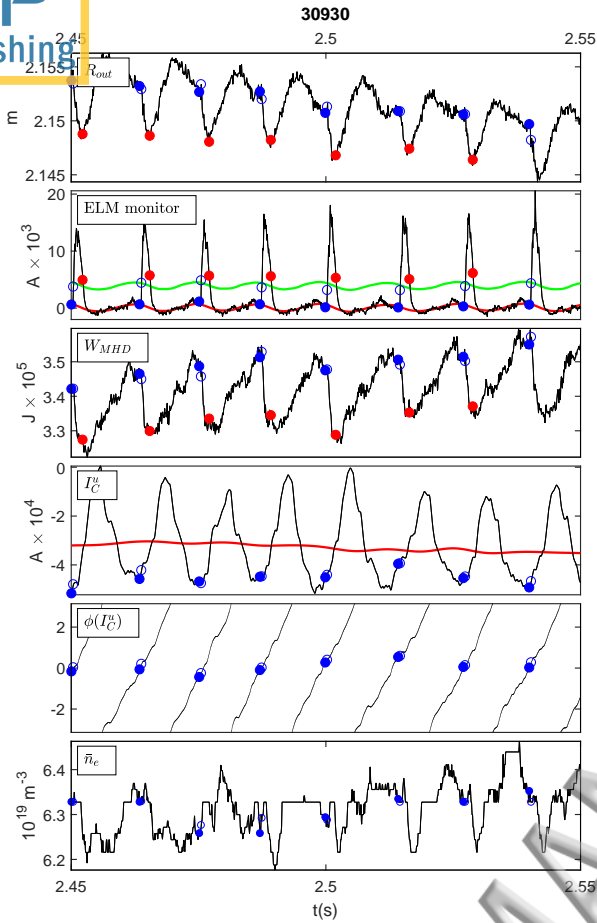
FIG. 8: Time traces plotted for a short time window of the same duration as in Fig. 1 at a time within the interval of synchronous dynamics in plasma 30930. Format is as in Fig. 1. This short time interval is indicated by the red bar in Figure 6 top panel.
