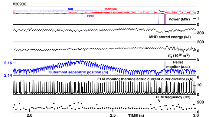
FIG. 5: Experimental plasma parameters for the early part of plasma 30930, in the same format as Fig.2. The plasma position is shifted during t = 2.0 - 2.6 s and at t = 2.75 s, the NBI beam drops shortly, changing the heating. Following this is the first of a sequence of injected pellets.
