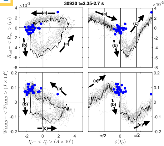
FIG. 14: Vertical control system current phase orders ELM cycle dynamics in plasma 30930. The format is the same as in the previous figure. The signals are plotted for the full interval of synchronous dynamics t = 2.35 - 2.7s . One cycle of this dynamics, from one ELM to the next, is overplotted (solid black line). All ELMs occurring in t = 2.35 - 2.7s are shown; for each ELM, the signals at the time t_B just before ELM onset are plotted (blue filled circles). The dynamics is a build up phase (a) terminating in ELM onset, followed by the ELM crash (b) and recovery (c).
