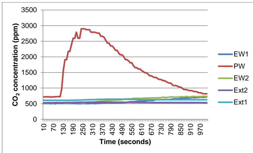
Figure 37 Test 4.10 CO 2 concentrations
