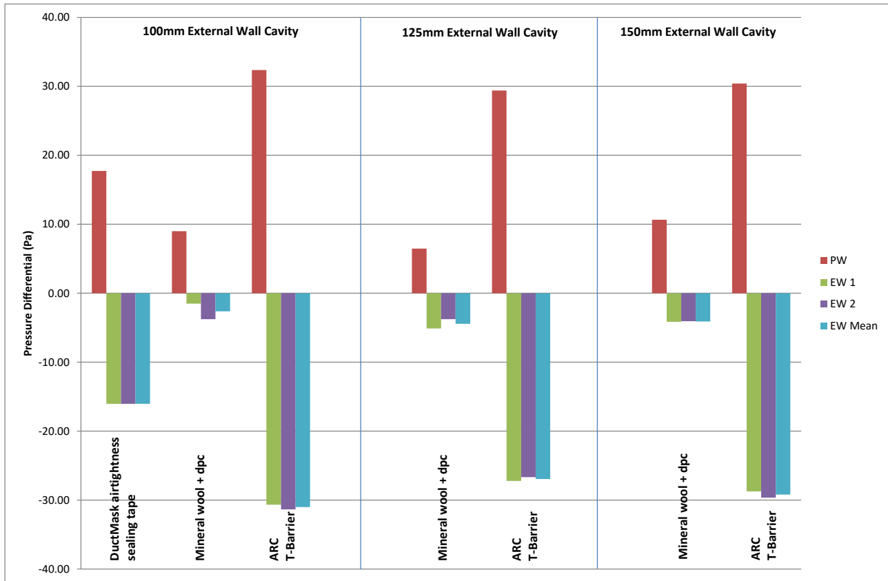
Figure 72 Pressure differentials: 100 mm party wall cavity at 250 l/min air input
