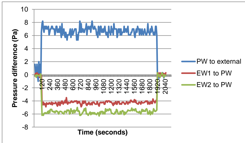
Figure 20 Test 1.4 Pressure differentials
