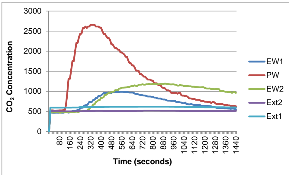
Figure 58 Test 4.17 CO 2 concentrations
