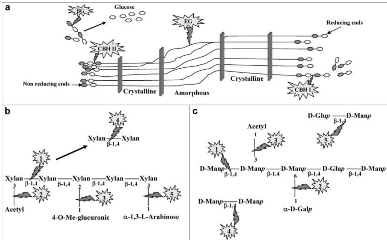
Fig. 4A–C. Enzymatic degradation of cellulose to glucose. CBHI Cellobiohydrolase I acts on the reducing ends; CBHII cellobiohydrolase II acts on the non-reducing ends; EG endoglucanases hydrolyze internal bonds. \beta -G \beta -Glucosidase cleaves the cellobiose disaccharide to glucose. B Enzymatic degradation of glucuronoxylans. 1 Endomannanase, 2 acetylxylose-esterase, 3 \alpha -glucuronidase. 4 \beta -xylosidase, 5 \alpha -arabinose (required only to hydrolyze glucuronoxylan from gymnosperms (see Fig. 2A). C Enzymatic hydrolysis of glucomannan. 1 Endomannanase, 2 \alpha -galactosidase (for gymnosperm hemicellulases, see Fig. 2B), 3 acetylglucomannan-esterase, 4 \beta -mannosidase, 5 \beta -glucosidase
