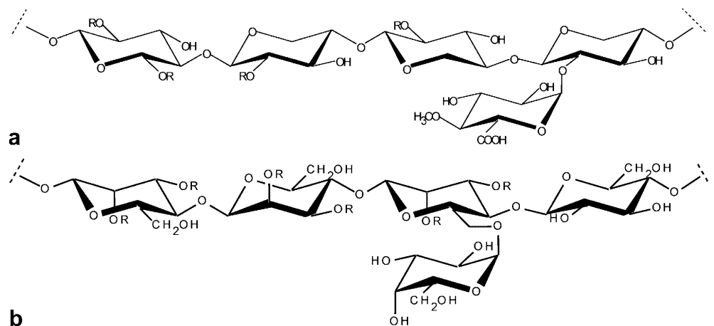
Fig. 2. A O-acetyl-4-O-methylglucuronoxylan from angiosperms. R H or acetyl group. Gymnosperm hemicellulose has the same basic structure but lacks acetyl groups and \alpha -1,3-l-arabinose residues. B O-acetyl-galactoglucomannan from gymnosperms. R H or acetyl group. Angiosperms contain lesser amounts of glucomannan, which always lacks \alpha -D-galactose
