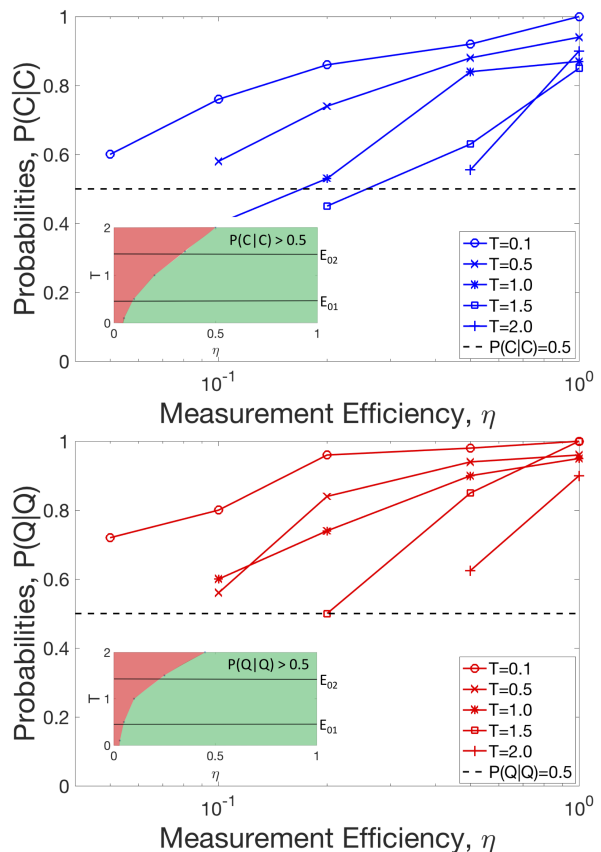
Figure 1. Numerically calculated probabilities for the identification of the correct dynamical evolution of optomechanical example with trapped nanoparticle in a double well potential: Q is calculated using a quantum SME, and C is calculated using the equivalent classical SDE. Probabilities p(C|C) and p(Q|Q) are shown, for different temperatures T as a function of the measurement efficiency \eta . Inserts show approximate regions where the models are distinguishable (green (light gray) shaded regions), as functions of temperature and measurement efficiency.
