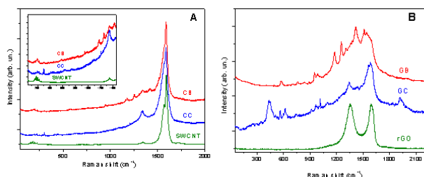
Figure 2. (A) Raman spectra of pristine SWCNT and its CC and CB hybrids in the range 50\text{--}2000\text{ cm}^{-1} and (B) Raman spectra of pristine rGO and its GC and GB hybrids.
