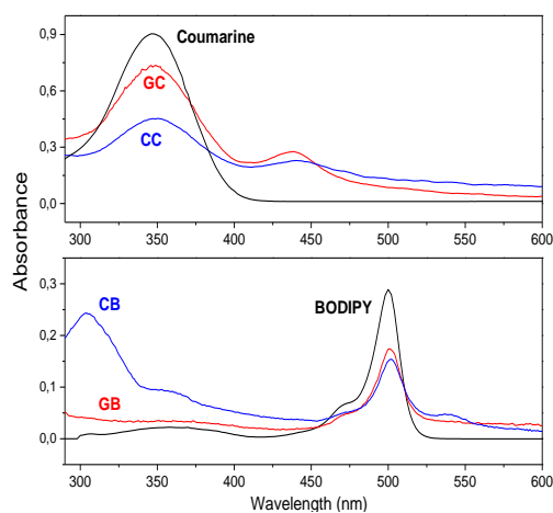
Figure 4. UV-Vis spectra of the compounds 2, 4 and their hybrids CB, CC, GB and GC.
