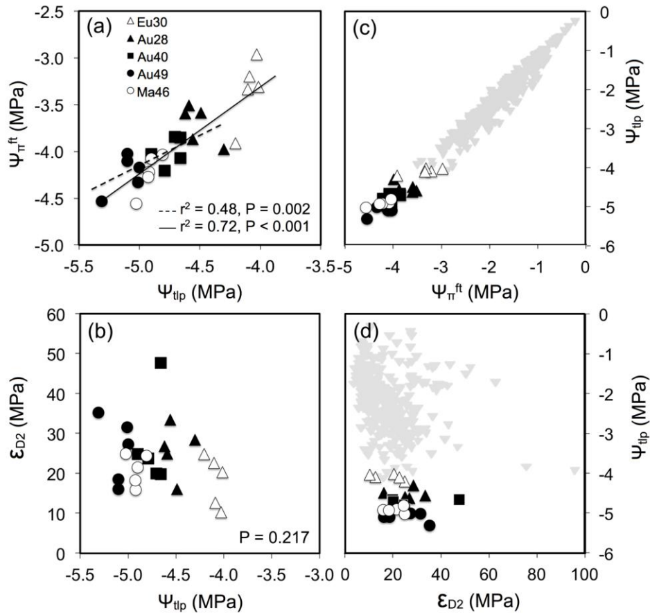
Figure 6. (a) Osmotic potential at full turgor ( \Psi_{\pi}^{ft} ) and (b) bulk modulus of elasticity ( \epsilon ) as functions of osmotic potential at the turgor loss point ( \Psi_{tip} ) when salinity was the source of variation in subsp. australasica (dashed line, black symbols) and when subspecies combined with environmental factors were the sources of variation (solid line, all symbols). Symbols as given in panel (a). Lines drawn by linear regression only for relationships with P \leq 0.05 . Data from panels (a) and (b) were replotted, respectively, in panels (c) and (d) relative to a global meta-analysis (Bartlett et al. , 2012).
