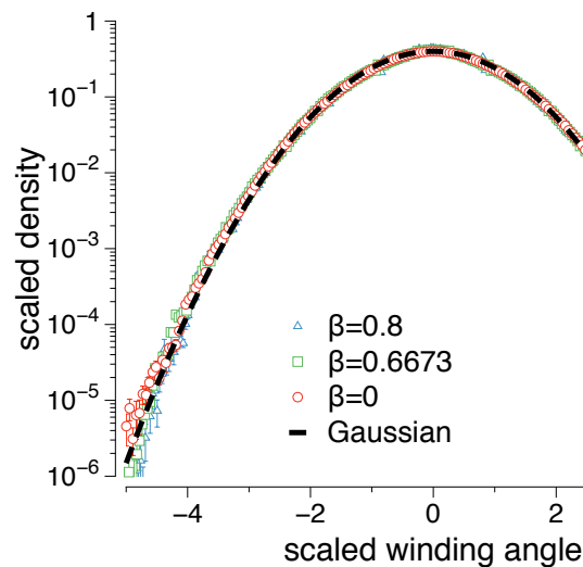
Figure 1: The scaled winding angle distribution for the ISAW model of polymer collapse with N = 1000 steps at \beta = 0 (swollen phase), \beta = 0.6673 ( \theta -point), and \beta = 0.8 (collapsed phase), demonstrating Gaussian behaviour at all temperatures.
