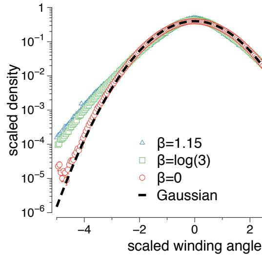
Figure 2: The scaled winding angle distribution for the ISAT model of polymer collapse with N = 1000 steps in the swollen phase, collapse point, and in the collapsed phase. While the swollen phase at \beta = 0 demonstrates the Gaussian form, the collapse point at \beta = \log(3) \approx 1.0986 and the collapsed phase at low temperatures (here \beta = 1.15 ) deviate substantially from this form.
