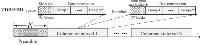
Fig. 6. A unified transmission scheme including preamble, uplink/downlink training and data transmission.
