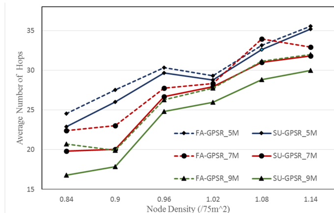
Fig. 6 Average Hop Counts
