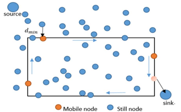
Fig. 2 Data Transmission Scenario in habitat monitoring WSN
