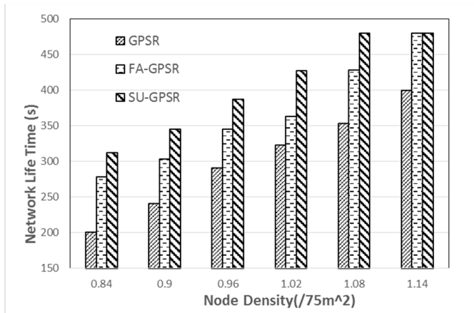
Fig. 4 Network Life Time with Various Network Size
