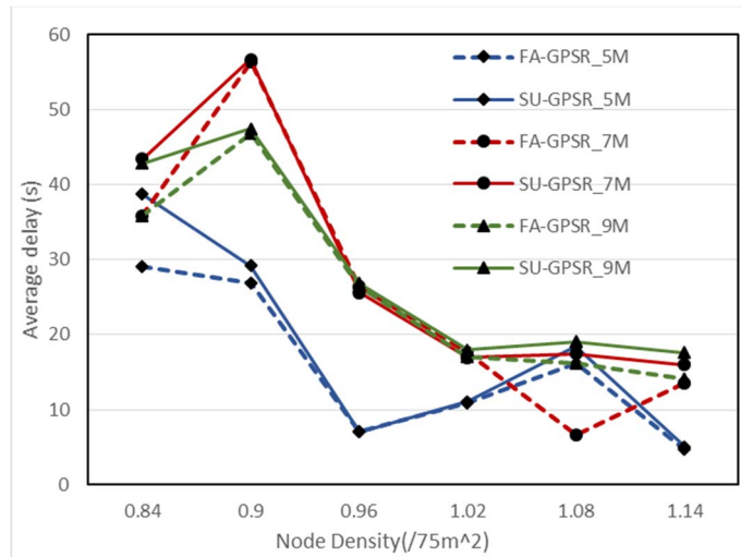
Fig. 5 Average End-to-End Delay with various Node Density
