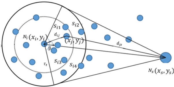
Fig. 1 The Division of the Forward Region [17]
