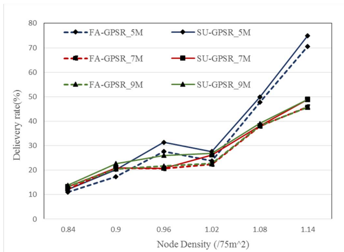
Fig. 7 Packet Delivery Successful Rate
