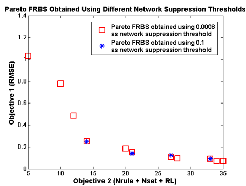
Fig. 12. Pareto FRBSs obtained using different \sigma .
