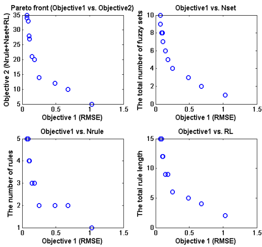
Fig. 7. The Pareto fronts obtained by using IMOFM_S.
