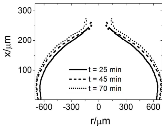
Figure 8. Radius of wetted region inside the textile vs x coordinates for \eta = 2.4 \cdot 10^3 Pa \cdot s .
