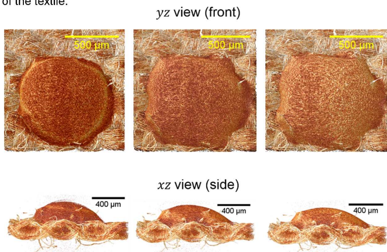
Figure 3. Tomography images showing the shape of the drop in the outside of the textile (online version in color). From left to right: t=25 mins, t=45 mins and t=70 mins, respectively. The liquid viscosity is \eta = 2.4 \cdot 10^3 \text{ Pa} \cdot \text{s} .
