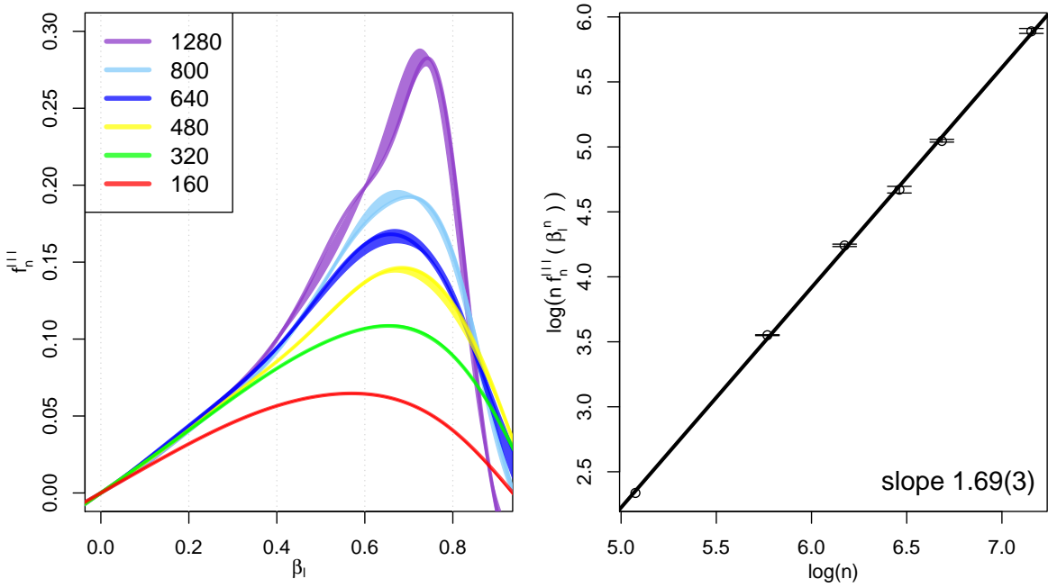
Figure 4.5. Left graph: Scaling of the third derivative of the free energy with respect to \beta_l at \beta_h = 2.5 . Right graph: Values of the maximum in n f'''_n(\beta_l^n) ( \beta_h = 2.5 ) against the length in log-log-scale, together with a linear fit indicating a slope of 1.69(3).
