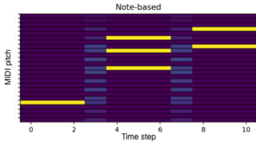
Figure 2. The prediction system output ( n_{\text{hidden}} = 256 , \text{learning\_rate}=0.01 ) with note-based time steps after going through the sigmoid, before thresholding. The ground truth is: E3, C4E4G4, F4A4. At each note change, a small probability is given to all notes in C major scale.
