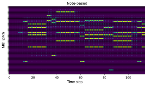
Figure 3. The output of the prediction system ( n_{\text{hidden}} = 256 , \text{learning\_rate}=0.01 ) with note-based time steps after going through the sigmoid, before thresholding. The ground truth is Chopin’s Prelude, No. 7, Op. 28 in A Major. At each eighth note, a small probability is given to some notes in A major, the tonality of the piece.
